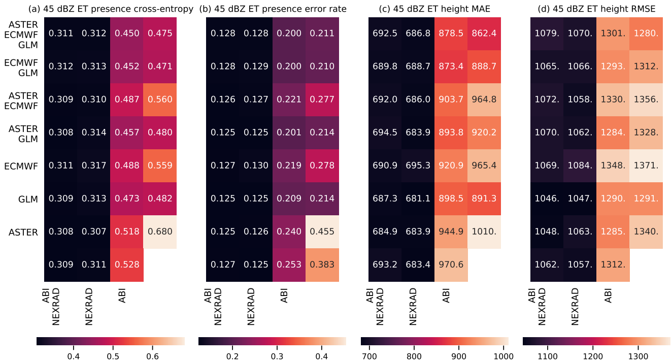
Figure 9. As Fig. 8, but for the ECHO45-OCC and ECHO45-HT predictands. In panel b, the bottom right corner shows the climatological occurrence. The results are shown for the 0–30 min time interval.
