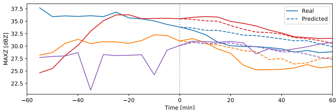
Figure 3. Examples of the prediction of MAXZ. The figure shows the curves of observed and predicted MAXZ for four different tracked centers. The solid lines show the development of MAXZ while the dashed lines show the predictions after t = 0 .
