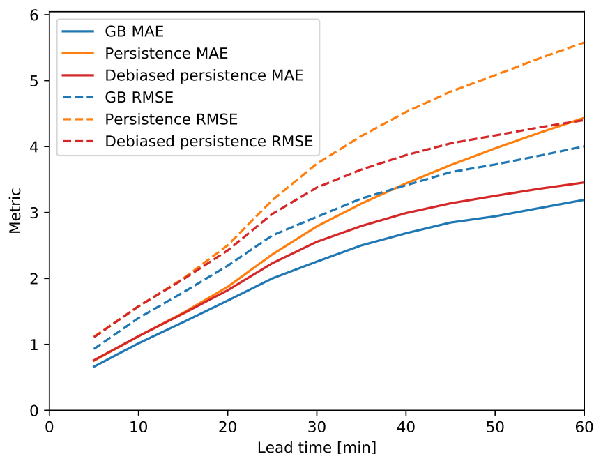
Figure 4. Errors in dBZ of the prediction of MAXZ as a function of lead time, using all the available data. The solid lines show the mean absolute error (MAE) while the dashed lines show the root-mean-square error (RMSE). The blue lines show the result from the GB tree, the orange lines show the Lagrangian persistence assumption and the red lines show the bias-corrected Lagrangian persistence.
