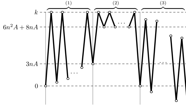
Fig. 4: Illustration of the sequence of energy difference changes on the folding pathway described in lines (1), (2) and (3). Details are discussed in the text of the paper.
