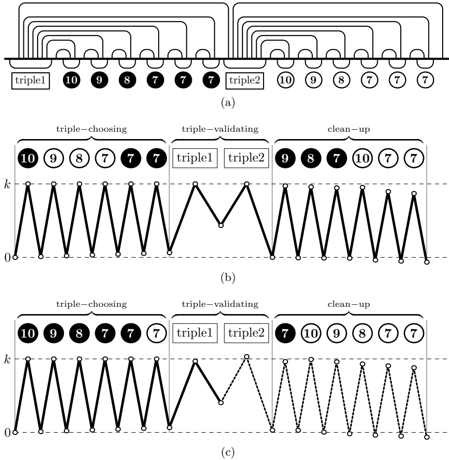
Fig. 5: Illustration of the construction in the proof of Theorem 2: (a) The instance created for the set of integers \{10, 9, 8, 7, 7, 7\} . (b) The energy function stays within the k barrier if the partition sets are selected correctly ( T_1 = \{10, 7, 7\} and T_2 = \{9, 8, 7\} ). (c) The energy function exceeds the barrier for an incorrect selection of partition sets ( T_1 = \{10, 9, 8, 7, 7\} and T_2 = \{7\} ). The dashed lines depict hypothetical progress of the pathway for some energy barrier larger than k .
