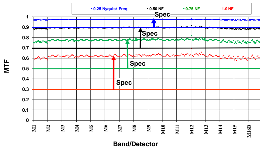
Figure 5. Ambient test result of the M-bands' MTF in track direction at 0.25, 0.5, 0.75 and 1.0 Nyquist frequencies (the straight lines denote the minimum requirements and the arrows denote the direction of compliance).
