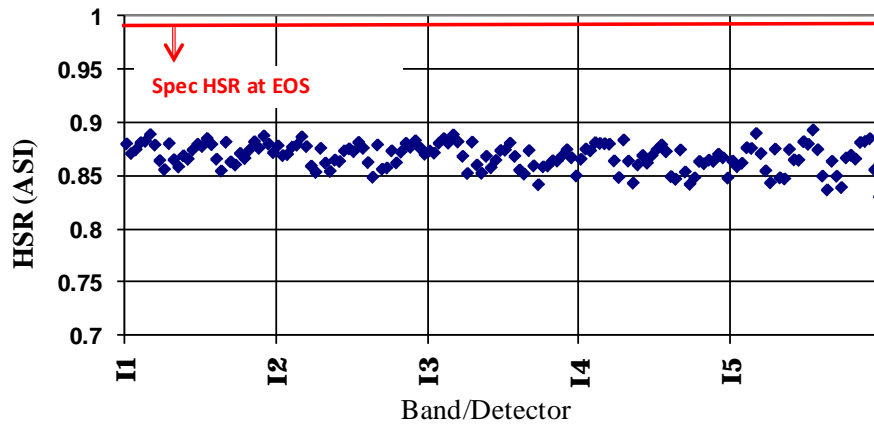
Figure 6. Ambient test result of the I-bands' HSR (the straight lines denote the minimum requirements and the arrow denotes the direction of compliance).
