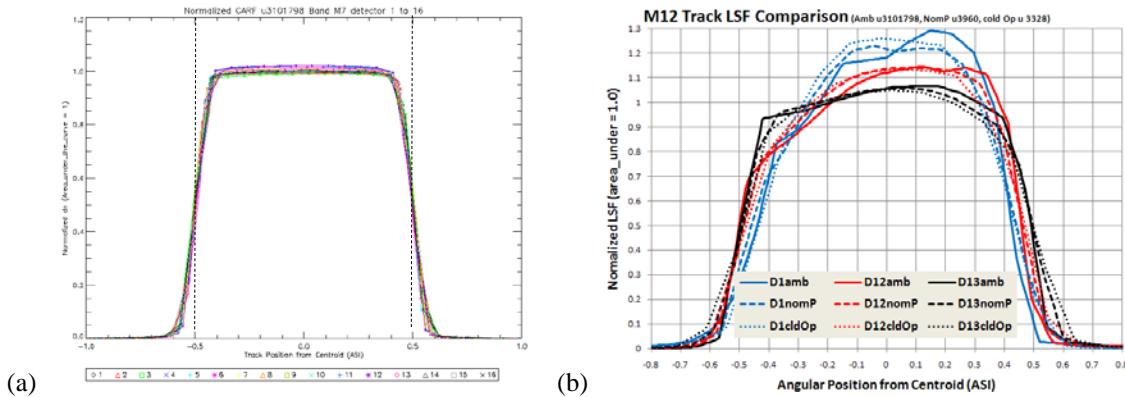
Figure 3. Example VIIRS LSFs: (a) Track static “nominal” LSFs for all detectors in band M7; (b) Anomalous LSFs for M12 detectors 1, 12 and 13.
