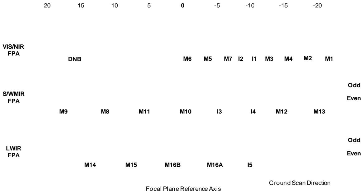
Figure 2. VIIRS focal plane assemblies and band layout in the scan direction 1 .
