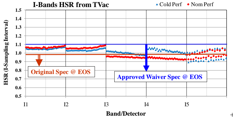
Figure 11. The I-bands scan HSR at the end of scan (EOS) from TVac cold and nominal performance plateaus.
