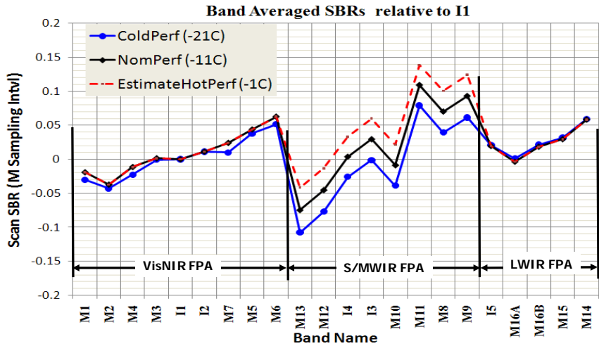
Figure 14. Averaged spectral band registration (SBR) in the scan direction from the TVac cold and nominal performance plateaus, and estimate from limited tests at the TVac hot performance plateau.
