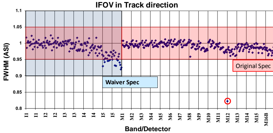
Figure 4. Ambient test result of I- and M-bands track IFOV. Each point represents an individual detector.
