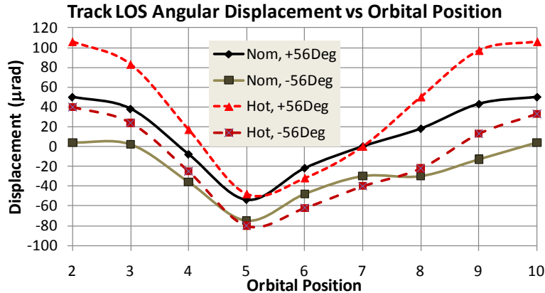
Figure 18. Examples of on-orbit track line-of-sight (LOS) pointing variation from STOP modeling at the nominal and hot performance plateaus for scan angles of +56 ° and -56 °.
