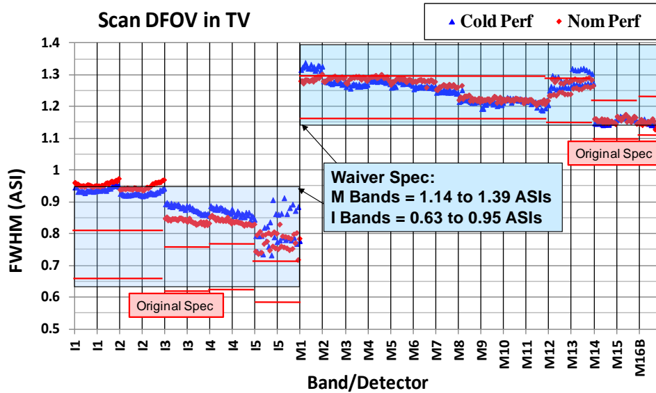
Figure 9. The I- and M-bands DFOV from TVac cold and nominal performance plateaus.
