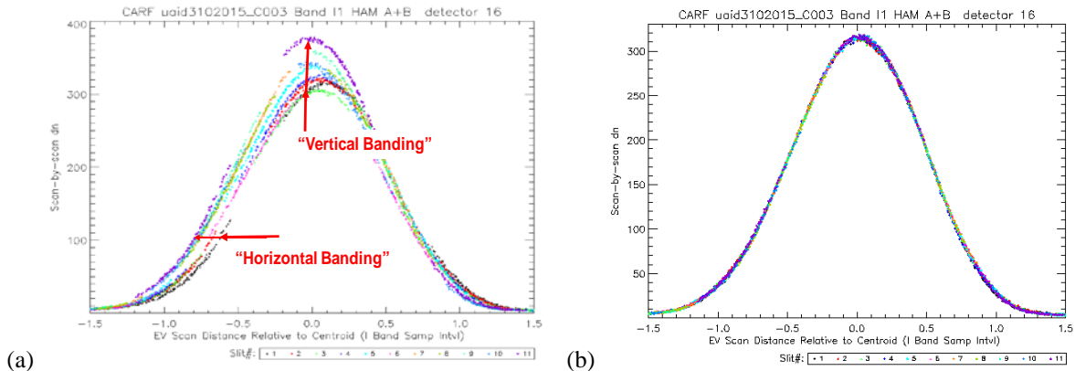
Figure 8. Scan direction DLSF for band I1 detector 16: (a) Original measurement with throughput and slit phase artifacts; (b) With throughput and phase corrections.
