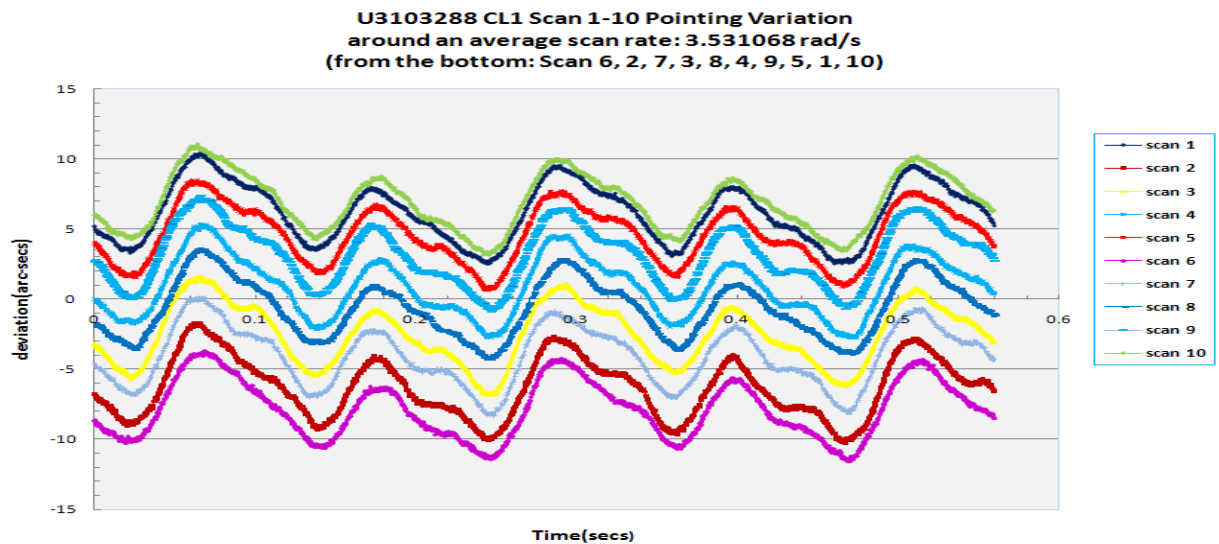
Figure 17. An example of pointing deviation from average scan rate and average bias in scan start positions. The curves will be followed closely with full complement of RTA/HAM encoder/timestamps information. This would be the pointing error in scan direction if the timestamps were lost (unlikely).
