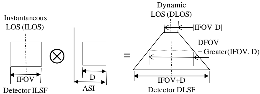
Figure 7. In the scan direction, the DLSF is a convolution of the detector ILSF with the integration drag.
