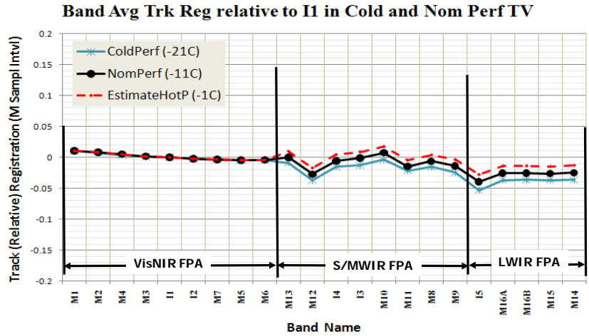
Figure 13. Results of averaged spectral band registration (SBR) in the track direction from the TVac cold and nominal performance plateaus, and estimate from limited tests at TVac hot performance plateau.
