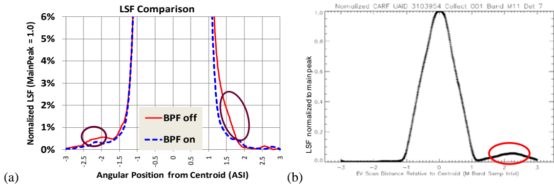
Figure 12. (a) Scan DLSF asymmetrical “high heel” on the right and sidelobe on the left in band M1; (b) Scan DLSF with a trailing sidelobe in band M11.
