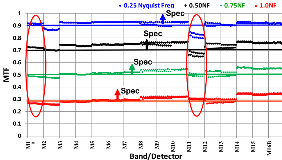
Figure 10. The M-bands scan MTF from TVac nominal performance plateau (M1* data is from a special test at hot performance plateau, see Figure 12(a)).
