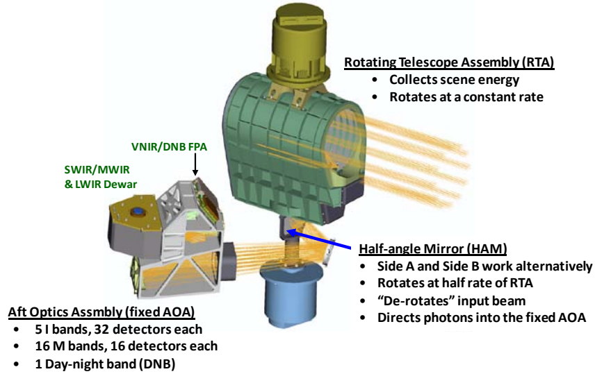
Figure 1. VIIRS optical system
