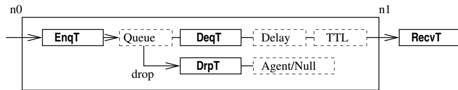
Figure 2.4: Tracing objects in a simplex link.
