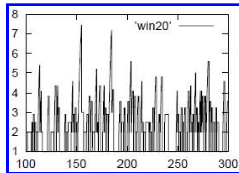
Figure 4.5: Window size of TCP with 20% random losses: a zoom.
