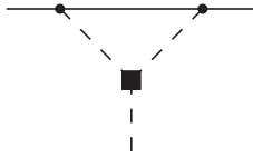
Figure 2. Correction to the g_1 pion-nucleon vertex induced by the CP-violating three-pion vertex in eq. (1.1). Notation as in figure 1.
