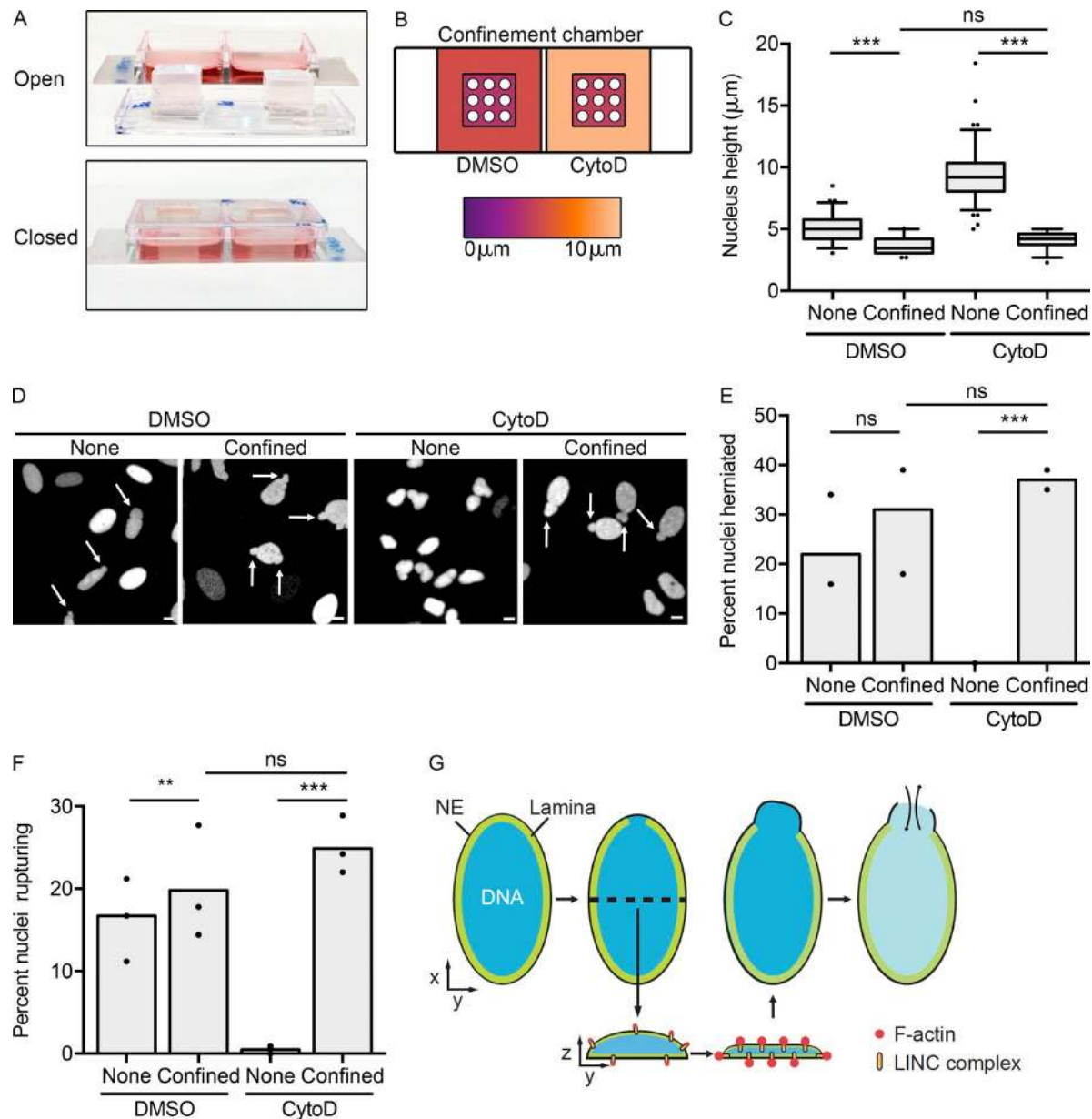
Figure 5. Mechanical confinement of U2OS nuclei is sufficient for NE rupture. (A) Images of cell confinement device. (B) Schematic representation of confinement device as viewed from objective. Large squares represent wells, small squares represent areas under the confinement slide, and circles indicate areas where pillars contact well bottom (not to scale). Colors represent mean nucleus height from C. (C) Quantification of nucleus height of U2OS GFP-LmnB1 cells treated with indicated drugs and confined for at least 1 h before imaging. Boxes are quartiles and whiskers are 5th to 95th percentiles. n \geq 60 nuclei; two-way analysis of variance, P < 0.001 for drug and confinement variables. **, P < 0.01 ; ***, P < 0.001 (multiple comparisons). (D) Images from 24-h time lapse of U2OS GFP-NLS shLmnB1 cells confined after treatment with indicated drugs. Arrows indicate sites of chromatin herniation. (E) Quantification of chromatin hernia formed during 24-h time-lapse imaging. Graph represents pooled data (columns) from two experiments (points, n > 150 cells). \chi^2 analysis P < 0.001 , results of Fisher's exact test between indicated pairs above the graph. ***, P < 0.001 ; ns, P > 0.05 . (F) Quantification of NE rupture during 24-h time-lapse imaging. Graph represents pooled data (columns) from three experiments (points, n > 150 cells). \chi^2 analysis, P < 0.001 , with results of Fisher's exact test between indicated pairs shown above the graph. **, P < 0.01 ; ***, P < 0.001 ; ns, P > 0.05 . (G) Model of interphase NE rupture in cultured cells. Bars, 10 \mu\text{m} .
