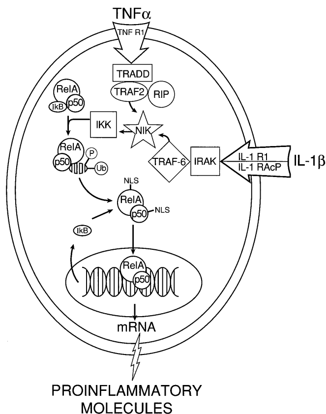
Fig. 1 TNF- \alpha binds to the type 1 TNF receptor (TNFR1), which results in an association with TNFR1-associated death domain protein (TRADD), the receptor-interacting protein (RIP), and the TNF receptor-associated factor-2 (TRAF-2). These cytoplasmic proteins form an active signalling complex that interacts with NF- \kappa B-inducing kinase (NIK). Activation of NIK results in phosphorylation of I \kappa B kinases (IKK), which cause phosphorylation I \kappa B. Phosphorylated I \kappa B is targeted for destruction by the ubiquitination/proteasome degradation pathway, allowing the translocation of NF- \kappa B to the nucleus. IL-1 \beta binds to the type 1 IL-1 receptor (IL-1R1) and the IL-1 receptor accessory protein (IL-1RAcP) which facilitates an interaction between IL1 receptor-associated kinase (IRAK) and TNF receptor-associated factor-6 (TRAF-6). These proteins form an active signalling complex that also results in activation of NIK and IKK leading to the sequence of events that results in activation of NF- \kappa B. Activation of NF- \kappa B results in expression of mRNA of a variety of pro-inflammatory mediators (see Table 1) which are involved in the pathogenesis of SIRS, MODS and ARDS. I \kappa B is also induced by NF- \kappa B activation and contributes to the down-regulation of this intracellular signalling cascade
