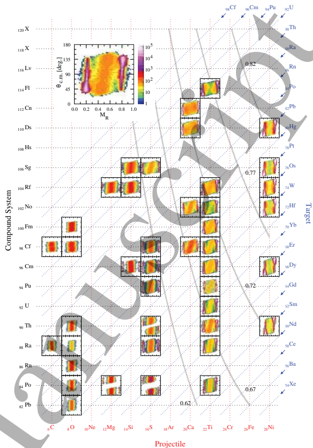
Figure 62. Fission-fragment mass-angle distributions (MADs)[131]. All miniatur plots have the same axes as the large MAD (top left, ^{48}\text{Ti} + ^{170}\text{Er} at E_{\text{beam}} = 225.0 MeV). The full gray lines correspond to the noted constant values of the effective entrance-channel fissility parameter x_{\text{eff}} [381]. The intensity scale represents counts per pixel in the MAD, proportional to d^2\sigma/d\theta_{\text{c.m.}}dM_R .
