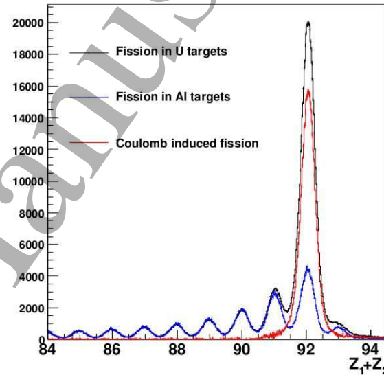
Figure 20. (Color online) Charge-sum Z_1 + Z_2 spectrum of the fission fragments produced in the aluminum targets (blue histogram) and in the uranium targets (black histogram) from a ^{238}\text{U} secondary beam in the SOFIA experiment. The blue histogram has been normalized in order to represent the fraction of nuclear-induced fission in the uranium targets at Z_1 + Z_2 = 92 . The difference spectrum (red histogram) is the deduced contribution from electromagnetically induced fission in the uranium targets. The figure is taken from Ref. [252].
