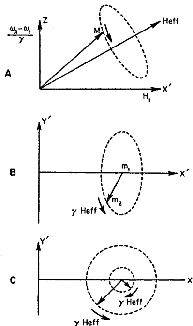
FIG. 1. (A) In the coordinate frame rotating with the frequency of the large radio-frequency field, the magnetic moment carries out a free precession about the effective field H_{\text{eff}} with an angular frequency \gamma H_{\text{eff}} . (B) The projection of this magnetic moment on the x'-y' axis of the rotating frame describes an ellipse. (C) This ellipse is decomposed into two components of different magnitudes rotating with the same angular frequency but in opposite directions.
