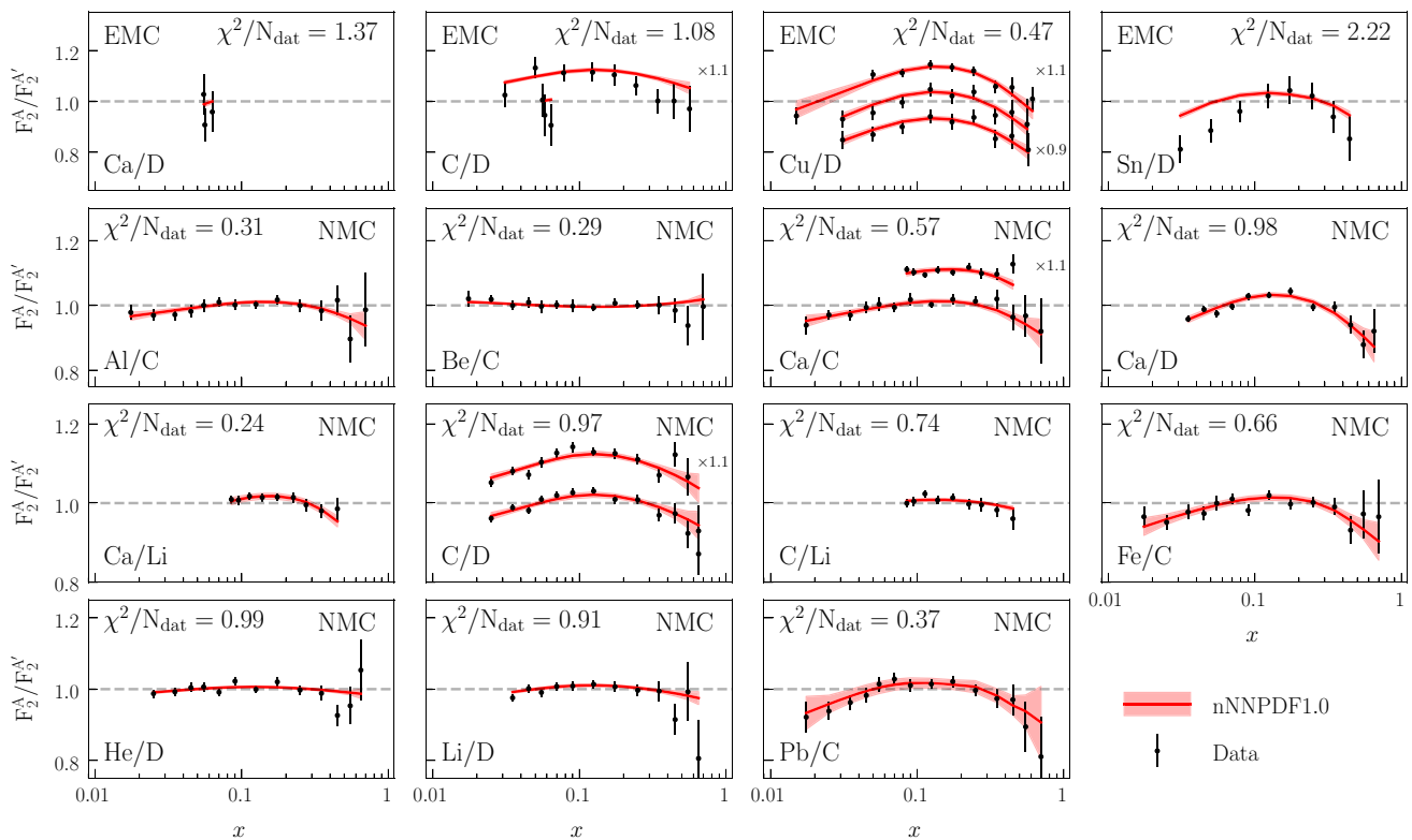
Fig. 13 Comparison between the experimental data on the structure function ratios F_2^A/F_2^N and the corresponding theoretical predictions from the nNNPDF1.0 NLO fit (solid red line and shaded band) for the measurements provided by the EMC and NMC experiments. The central values of the experimental data points have
