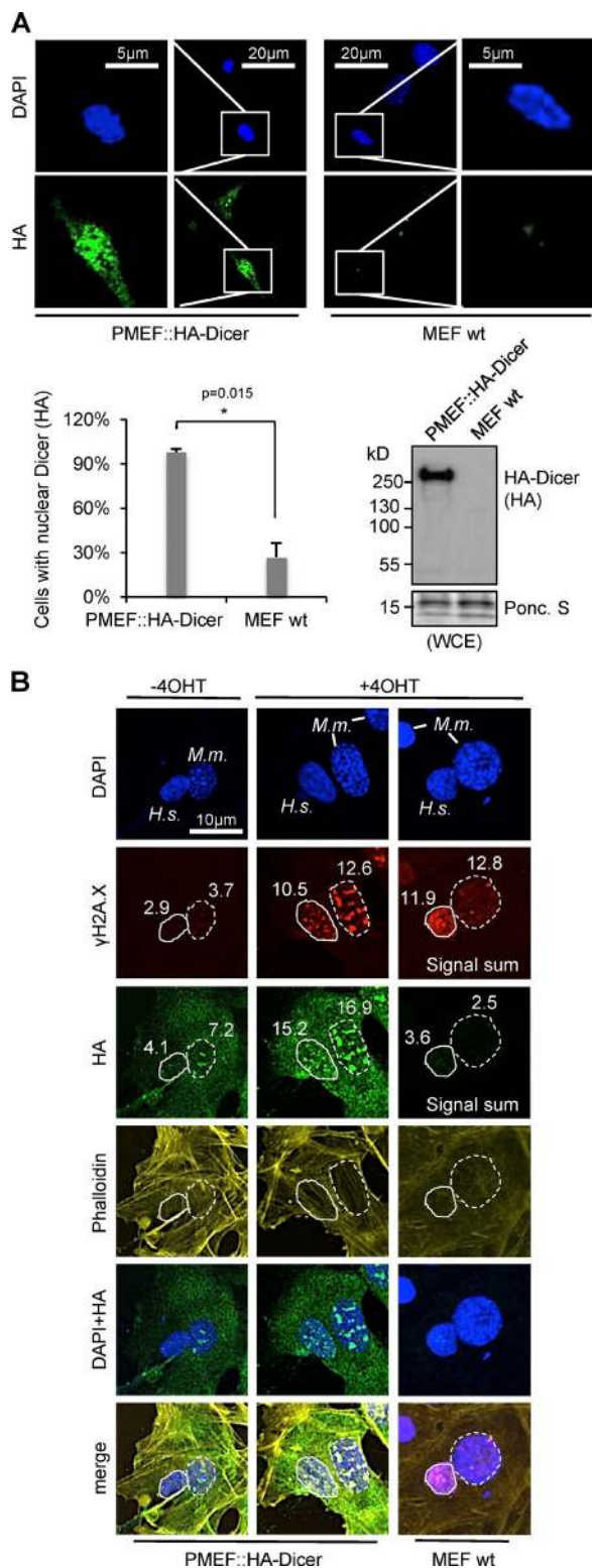
Figure 4. Accumulation of mouse HA-Dicer in damaged nuclei. (A) Confocal imaging (top) detecting endogenously tagged, mouse HA-Dicer in primary MEF cell line PMEF::HA-Dicer. Control, MEF wild type. Quantitation as the percentage of cells with nuclear HA signal. n > 50 (bottom left). *, P < 0.05 ; error bars, means \pm SEM of three biological replicates and immunoblot detecting HA-Dicer (bottom right). WCE, whole cell extract; Ponceau S staining, loading control. (B) Confocal imaging of heterokaryon fusions between human AsiSI-ER U2OS cells and mouse PMEF::HA-Dicer or
