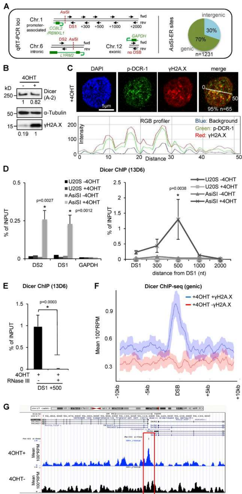
Figure 2. Recruitment of Dicer to DNA double-strand breaks in AsI/ER U2OS cells. (A) Structure of genomic loci assessed by quantitative RT-PCR (left) and genome-wide AsI/ER target site distribution; n, number of predicted AsI/ER target sites (right); fwd/rev, forward/reverse. (B) Immunoblots detecting total Dicer (A-2) and \gamma H2A.X after induction of DNA double-strand breaks (DSBs). 4OHT, 4-hydroxytamoxifen. Immunoblots were quantified using ImageJ. (C) Confocal imaging of phosphorylated Dicer (p-DCR-1) and \gamma H2A.X (top). All quantifications represent number of cells exhibiting shown phenotype. Quantification using ImageJ RGB profiler (bottom). (D) ChIP analysis showing Dicer occupancy at DSBs DS1/2 in wild-type and AsI/ER U2OS cells using site-specific primers. GAPDH, control locus. *, P < 0.05 ; error bars, means \pm SEM of three biological replicates. (E) ChIP analysis showing Dicer occupancy at DS1 in absence or presence of recombinant RNase III preincubation. *, P < 0.05 ; error bars, means \pm SEM of three biological replicates. (F) ChIP-seq signal upon +4OHT incubation at 200 \gamma H2A.X-positive/negative genic sites after removal of duplicate reads. A rolling mean of 1 kb was applied after removal of 2% of the top and bottom values. Shadow, rolling SD. (G) Snapshot showing Dicer binding at genic AsI/ER target site upstream of TRIM37 before (4OHT - ) and after (4OHT + ) DNA damage. Red box, proximal region to AsI/ER site.
