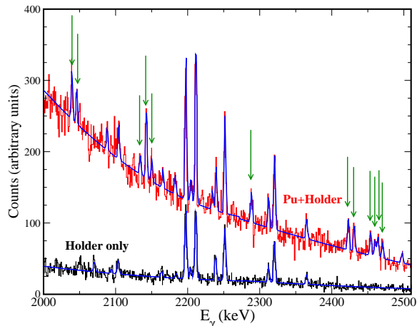
FIG. 3: Histograms of the measured spectra for the ^{239}\text{Pu} measurements. The upper histogram is a compilation of two data runs in two different configurations (Pu target and holder). The lower histogram is the background (holder only) spectrum from one run. Both data sets include Al calibration target. The arrows indicate peaks attributed to ^{239}\text{Pu} . A smooth curve is overlaid on both histograms to aid the eye.
