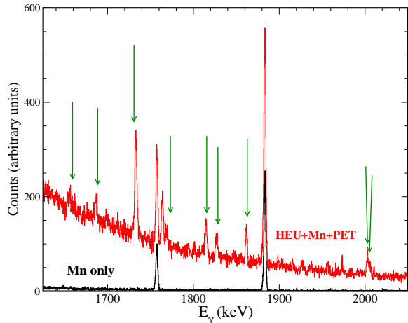
FIG. 2: Histograms of the measured spectra for the ^{235}\text{U} measurements. The top spectrum is for the HEU+Mn+PET plastic container. Arrows indicate peaks attributed to ^{235}\text{U} . The bottom spectrum is for Mn only. The relative scale of the Mn only spectrum to the HEU+Mn+PET spectrum is arbitrary. The peak at 1764 keV not attributed to Mn or ^{235}\text{U} is from ^{214}\text{Bi} radioactive decay.
