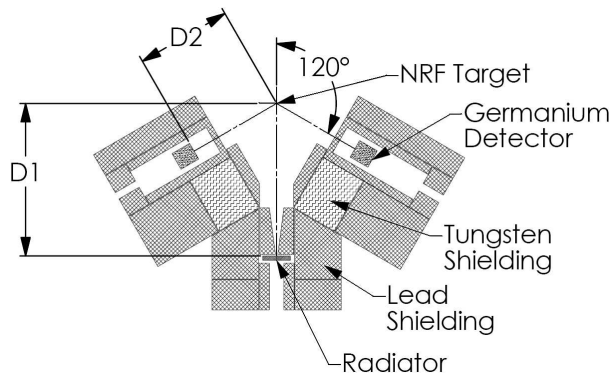
FIG. 1: NRF setup at the HVRL at MIT. See text for details.
