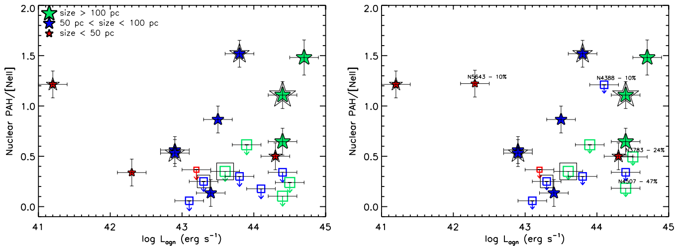
Figure 5. Flux ratio of the 11.3 \mu\text{m} PAH and the [Ne II] lines plotted against the AGN luminosity for the total (AGN+SF) [Ne II] emission (left) and corrected when possible for the AGN contribution (right panel), using values from Meléndez et al. (2008) (these are shown with name tags on the figure, with the corresponding percentage of star formation). See the text for details.
