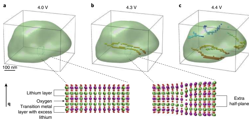
Fig. 1 | Formation of a dislocation network during charge. Isosurface rendering of a LRL0 particle measured in operando during charge. a , At a charge state of 4.0 V versus \text{Li}^+ no dislocations are observed in the particle. The inset shows a schematic of a dislocation-free crystal. b , At 4.3 V two edge dislocations have formed during lithium extraction (shown by small spheres in the particle). The inset shows a schematic of an edge dislocation. c , At 4.4 V a dislocation network emerges (colours are used to represent different dislocations). The direction of the X-ray scattering vector \mathbf{q} (perpendicular to the layers) is indicated and the size of the particle is around 300 \times 300 \times 500 \text{ nm}^3 .
