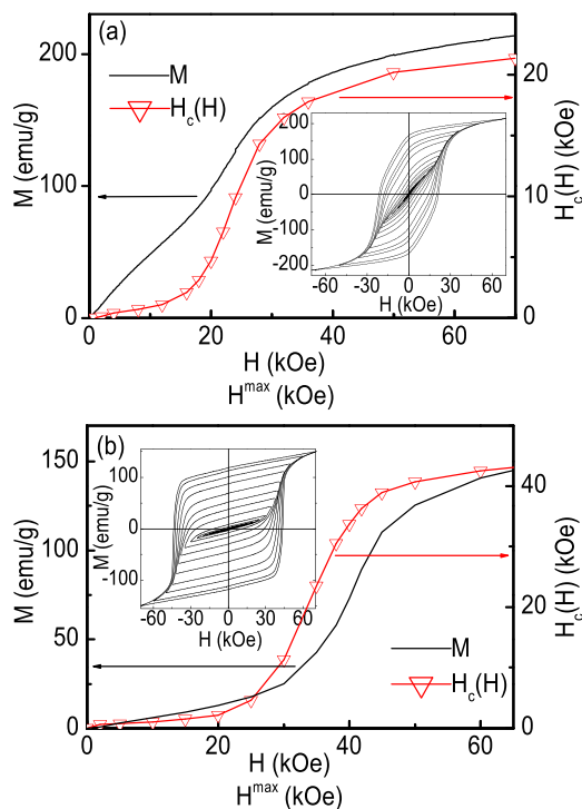
FIG. 4. Initial magnetization curve and field dependence of coercivity for \text{Pr}_8\text{Fe}_{87}\text{B}_5 (a) and for \text{Pr}_{12}\text{Fe}_{82}\text{B}_6 ribbons (b) at a temperature of 60 K, and the insets show minor hysteresis loops for \text{Pr}_8\text{Fe}_{87}\text{B}_5 (a) and for \text{Pr}_{12}\text{Fe}_{82}\text{B}_6 ribbons (b).
