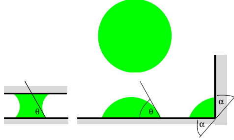
Figure 1: Schematics of critical nuclei in the bulk, on a flat surface, in a 90^\circ corner or wedge, and in a slit pore. The first three are nuclei of a new bulk phase and are at the same value of the supersaturation. The nucleus in the pore (on the left) is at a lower chemical potential. The transition in the pore is shifted by the interaction with the walls of the pore to lower values of the chemical potential. The contact angle \theta is indicated on the nuclei on the flat surface and in the pore. We specify wedge angles via the angle \alpha , which here is 45^\circ . The internal angle, here 90^\circ , equals 180^\circ - 2\alpha . Note that the radius of curvature of all the critical nuclei except the one in the pore is the same as it is set by the supersaturation via (4). The nucleus for homogeneous nucleation is a sphere whilst those for heterogeneous nucleation on flat surfaces and in wedges are parts of spheres of the same radius. The schematics are two-dimensional cross-sections through three-dimensional nuclei.
