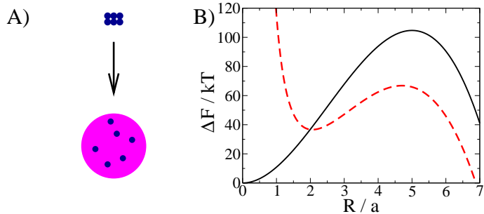
Figure 5: A) A schematic of nucleation occurring on a cluster of molecules. These attract each other strongly in the bulk phase, and so form a compact cluster there, but are highly soluble in the nucleating phase. At the top is shown the tightly bound cluster of 6 impurity molecules in the bulk phase. They are shown as small blue circles. Below is shown a nucleus (magenta) of the new phase, with the 6 impurity molecules diffusing inside it. B) A plot of the free energy of a nucleus as a function of its radius R . The solid black curve is for homogeneous nucleation within the standard CNT (2). The red dashed curve is for nucleation on n = 10 soluble impurity molecules. The free energy plotted is that of (17) but with \Delta F_{\text{SOL}} subtracted off. The parameter values are \rho_n = 1/a^3 , \gamma = kT/a^2 , B_2 = 4a^3 and \Delta\mu/kT = 0.4 .
