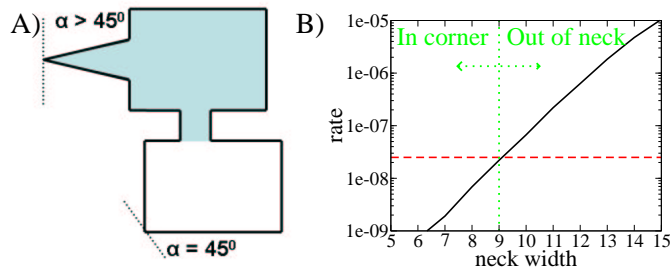
Figure 4: A) A schematic of a simple model of a porous medium. Porous media consist of interconnected networks of pores. Our model consists of only two, interconnected, pores. The top pore is shown filled with the liquid phase, which is shown in light blue. Corners are defined by their values of \alpha . This is shown explicitly for a right-angled corner and for a corner in a narrow wedge. B) A plot of nucleation rates as functions of neck width. The black curve is for nucleation out of a neck, and the red dashed curve is for nucleation in a corner. The model is the two-dimensional Ising model, and the contact angle between the nucleating phase and the walls \theta = 90^\circ . The rates are from [15]. The vertical dotted green line separates the region where nucleation out of the neck is faster and so dominates from the region where nucleation in the corner is faster and so it dominates.
