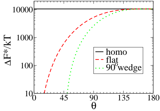
Figure 3: Classical nucleation theory predictions for the nucleation barrier \Delta F^* as a function of the contact angle \theta between the nucleating phase and a surface. The solid line is the barrier for homogeneous nucleation, the red dashed curve is for heterogeneous nucleation on a smooth flat surface, and the dotted green curve is for heterogeneous nucleation in a right-angled wedge, \alpha = 45^\circ . We took \gamma = kT/a^2 , \rho_n = 1/a^3 and a supersaturation \Delta\mu/kT = 0.04 . Here a is the size of the molecules which provides the microscopic lengthscale but whose value does not effect the barrier height.
