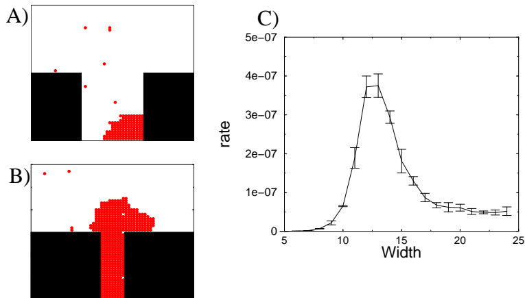
Figure 2: A) and B) are snapshots of critical nuclei for nucleation in a pore and out of a pore, respectively. C) is the rate of nucleation as a function of pore width in lattice sites. The rate is for a single pore and is per simulation cycle. A cycle is one attempted spin flip per spin. The error bars are the standard deviations of the rates obtained in 4 independent runs. The model is the two-dimensional Ising model with parameters J/kT = 0.8 and h/kT = 0.05 [15]. The systems are 60 by 60 lattice sites in size and the pores are 30 sites deep and have fixed spins along both sides and the bottom. In A) and B) the fixed spins are shown in black, while the up spins are red. The sites with down spins are left white. It is the up-spin phase that is nucleating from the down-spin phase. The pore in A) is 9 lattice sites across and that in B) is 24 sites across. A) and B) are from figure 1 of [15] and C) is from figure 3 of [15].
