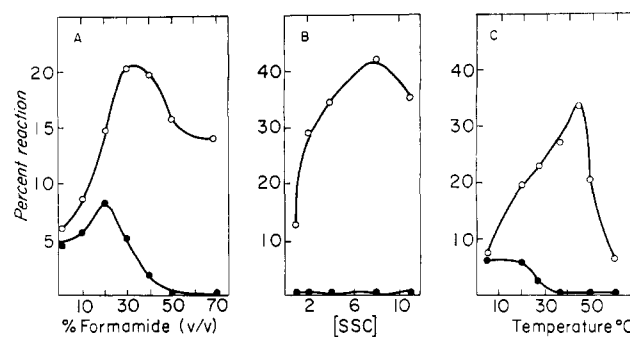
FIGURE 2: Extent of reaction and specificity of DNA-DNA duplex formation in formamide; 1.2 \mu\text{g} of denatured, ^3\text{H} -labeled B. subtilis DNA (9100 cpm) was incubated in 0.2 ml of solvent with 12 \mu\text{g} of filter-bound B. subtilis DNA, or 14 \mu\text{g} of filter-bound rabbit DNA, for 22 hr, at conditions described below. At the end of the reaction, the filters were washed for 3 min in 5 ml of the solvent and at the temperature of reaction, and then for 3 min in 5 ml of 2 \times SSC to remove the formamide. Per cent of labeled input DNA bound is plotted for the homologous B. subtilis DNA ( \circ ) and heterologous rabbit DNA ( \bullet ) filters. (a) Extent of reaction at 20^\circ in 2 \times SSC with various concentrations of formamide. (b) Extent of reaction at 37^\circ in 30% formamide at various concentrations of SSC. (c) Extent of reaction in 2 \times SSC and 30% formamide at various temperatures.
