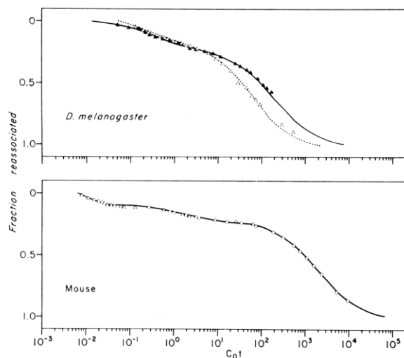
FIGURE 6: The renaturation kinetics of D. melanogaster DNA and mouse DNA. The rate of renaturation of denatured D. melanogaster DNA in SSC at 60° (▲) or 5 × SSC containing 48% formamide at 37° (△) was followed as described in Figure 5. The rate of reassociation of denatured mouse DNA was measured in 5 × SSC containing 48% formamide at 37° at two concentrations in cuvettes with different light paths: 50 µg/ml, 1-cm light path (△) and 500 µg/ml, 1-mm light path. The initial 10% which represents the mouse satellite, reassociated before the temperature was equilibrated at 37°. The rate of renaturation for the remaining 90% is plotted on curves which represent ideal second-order kinetics for a 15% component (redundant sequences) and a 75% component (unique sequences).
