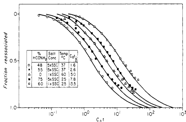
FIGURE 5: The rate of renaturation of sheared denatured B. subtilis DNA as a function of temperature and the concentration of salt and formamide. The DNA was denatured at a concentration of 50 \mu\text{g}/\text{ml} in a recording spectrophotometer and the rate of renaturation under the conditions shown in the inset was followed by the hypochromicity at 270 \text{m}\mu . The fraction of DNA reassociated, plotted as a function of the initial concentration (moles of P per liter) multiplied by the time (seconds). The data obtained are plotted on curves representative of theoretical second-order reactions.
