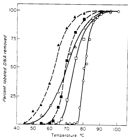
FIGURE 4: Thermal dissociation profiles of duplexes formed by incubating 1.2 \mu\text{g} of ^3\text{H} -labeled, sheared, denatured L-cell DNA with 12 \mu\text{g} of mouse DNA or hamster DNA bound to filters. The reactions were carried out at 45° for 16 hr in 0.2 ml of 1 \times SSC containing various concentrations of formamide. The amount of formamide used and the extent of reaction are as follows. (a) Mouse DNA: \Delta , 8% formamide, 10.3% reaction; \square , 25% formamide, 6.4% reaction; \circ , 50% formamide, 2.0% reaction. (b) Hamster DNA: \blacktriangle , 8% formamide, 3.7% cross-reaction; \blacksquare , 25% formamide, 0.88% cross-reaction. There was no measurable cross-reaction with hamster DNA in 50% formamide. Filters were washed in 5 ml of the incubation medium at 45° and then in 5 ml of 1 \times SSC. Dissociation of the duplex was accomplished by heating the filters to increasing temperatures. A filter was removed and counted at each indicated temperature.
