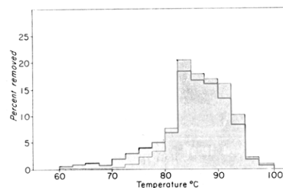
FIGURE 7: Thermal dissociation profiles of B. subtilis or D. melanogaster complexes by hydroxylapatite chromatography. The incubation mixture contained 30 µg/ml of 14 C-labeled B. subtilis DNA (120 cpm/µg) and 600 µg/ml of 3 H-labeled D. melanogaster DNA (10 cpm/µg). The DNA was sheared and denatured prior to incubation in 60% formamide-0.30 M phosphate buffer at room temperature for 5000 hr. This corresponds to a C_{0t} value of 32,000 for D. melanogaster DNA and 1600 for B. subtilis DNA. The sample was then diluted 60-fold in 0.12 M phosphate buffer (pH 6.8) and adsorbed to a 3-ml hydroxylapatite column. The column was washed twice with 5-ml aliquots of the phosphate buffer. The temperature of the column was raised in 2.5° increments and washed twice at each temperature. The DNA eluted at each temperature was collected by precipitation with trichloroacetic acid and counted. The shaded area represents the profile for B. subtilis DNA.
