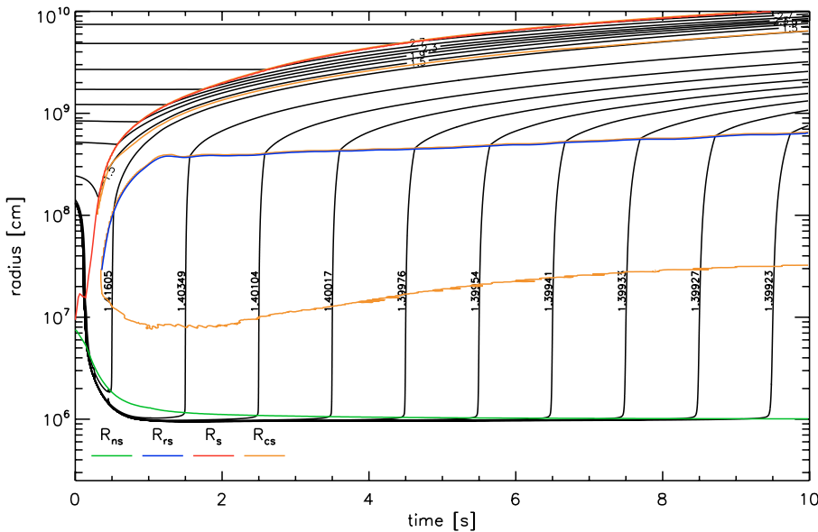
Fig. 3. Mass shell plot for the evolution of model M15-11-r1. The explosion occurs about 0.2 seconds after bounce. The red line marks the supernova shock, the blue line the wind termination shock, the orange lines the locations where the expansion velocity of the gas equals the local sound speed (sonic points), and the green line the neutron star radius defined as the location where the density drops below 10^{11} \text{ g cm}^{-3} . A contact discontinuity separates the dense shell of ejecta that were accelerated by the outgoing shock from the very dilute neutrino-driven wind. Mass shells in the wind are labelled by the corresponding enclosed baryonic masses.
