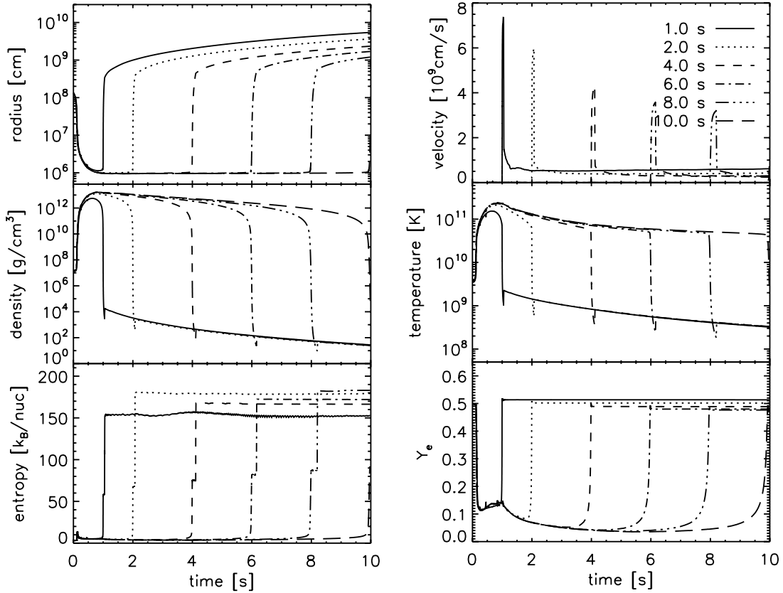
Fig. 6. Radius, density, entropy (left, from top to bottom), velocity, temperature, and electron fraction Y_e as functions of time along the trajectories of different mass shells that are ejected in the neutrino-driven wind of model M15-11-r1. The times correspond to the moments when the mass shells cross a radius of 100 km. After a very rapid expansion, the wind is abruptly decelerated by the termination shock. This leads to an increase of the entropy by more than a factor of two, and to a subsequently much slower decline of the temperature and density.
