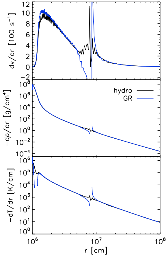
Fig. 1. Derivatives of the velocity ( top ), density ( middle ), and temperature ( bottom ) as functions of radius from our hydrodynamic model M15-11-r1 at 1.5 s after bounce (black lines) compared to these derivatives as computed from the relativistic stationary wind equations of Eqs. (5)–(7) in Thompson et al. (2001) (blue curves). These equations were evaluated by using the values of all gas quantities as provided by our hydrodynamic model. Consistency between our hydrodynamics results (with approximative treatment of relativity) and the fully relativistic wind solution would require the corresponding lines to lie on top of each other. The agreement is very good and the sonic point is located at about 80 km in both cases. This location is a critical point of the wind equations, which explains the pathological behavior of the curves there. The evaluation of the expression for the temperature gradient is numerically inaccurate in a region where the two terms in Eq. (7) of Thompson et al.’s paper are very large and have opposite signs, in which case dT/dr becomes slightly positive while the hydrodynamical result is still negative.
