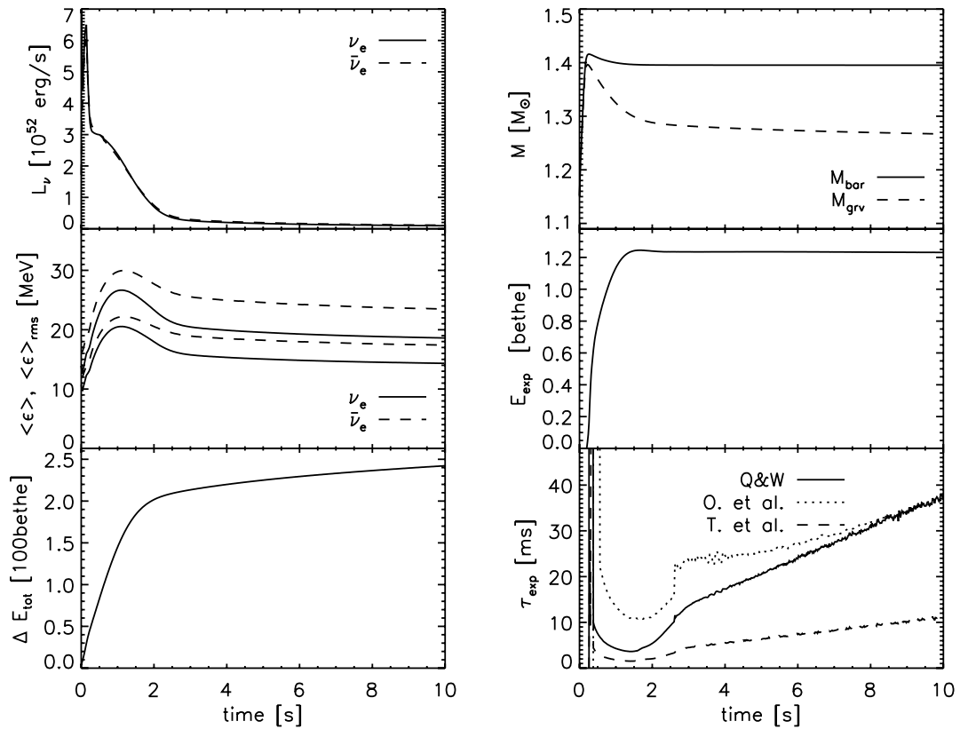
Fig. 12. Same as Fig. 4, but for model M15-lt1-r4. Compared to model M15-l1-r1, the neutrino luminosities and mean energies decrease faster, the total energy radiated in neutrinos and the explosion energy are lower, and the gravitational mass of the neutron star is larger. The breeze solutions that develop between 2.5 s and 7 s have significantly longer expansion timescales.
