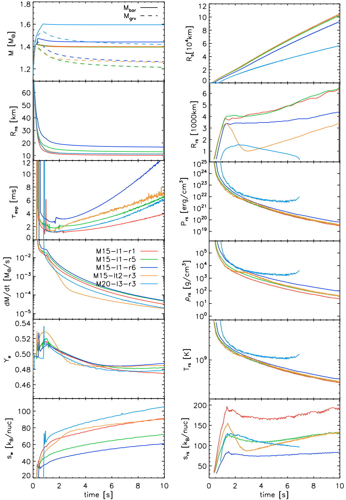
Fig. 10. The same as Fig. 8, but for simulations with varied inner boundary conditions. The models M15-11-r5, M15-11-r6, M15-1t2-r3, and M20-13-r3 are compared with our reference 15 M_{\odot} model M15-11-r1 in order to demonstrate the influence of different neutron star radii, neutron star masses, and core neutrino luminosities at the inner grid boundary.
