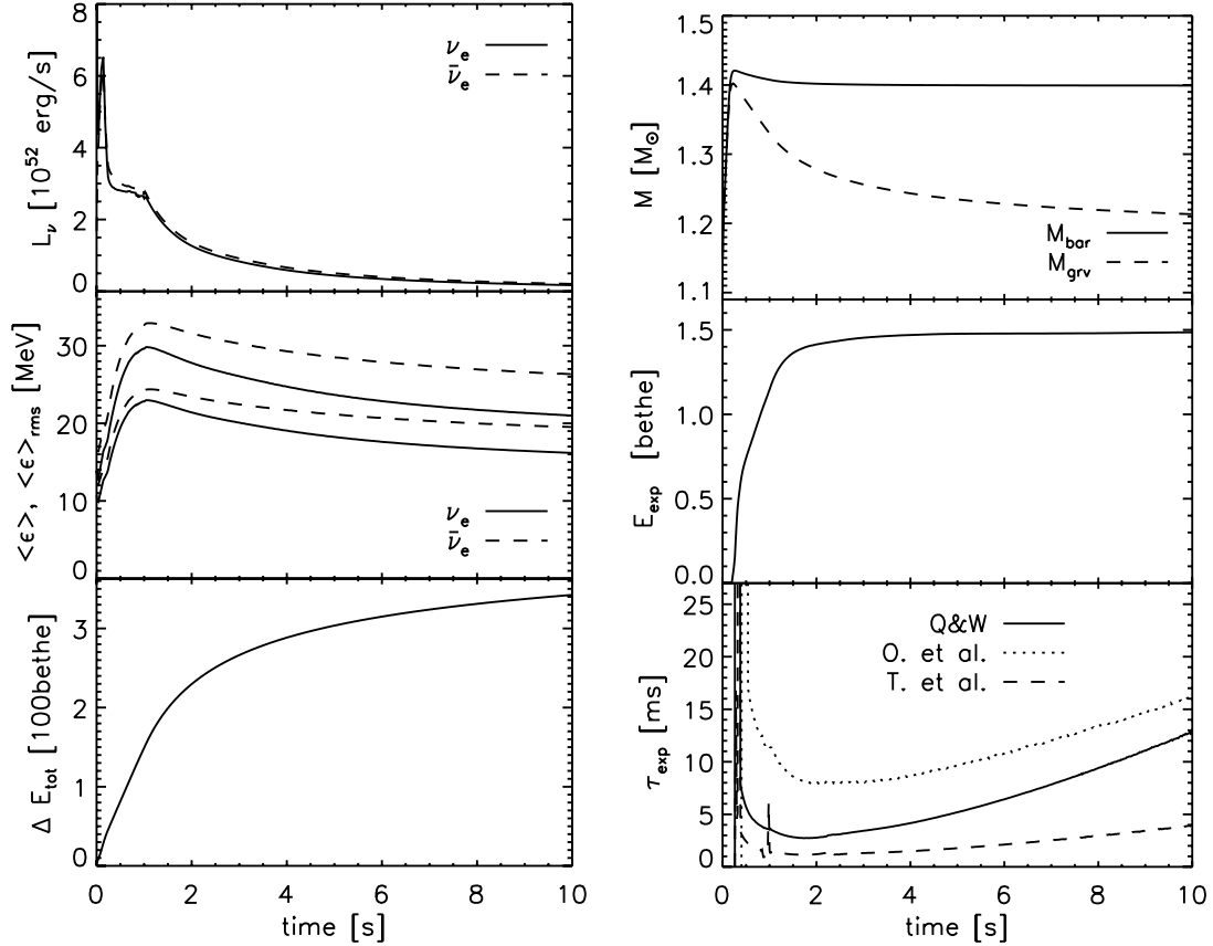
Fig. 4. Luminosities, mean energies according to Eq. (8), and rms energies (Eq. (9), \langle \epsilon \rangle_{\text{rms}} > \langle \epsilon \rangle ) of \nu_e and \bar{\nu}_e , and total energy radiated in neutrinos of all flavors for model M15-11-r1 as functions of time ( left ), measured outside of the nascent neutron star (at a radius of 500 km). Note that we do not include gravitational redshifting in our neutrino treatment. The rapid decline of the luminosities after about 0.2 marks the end of the accretion phase of the forming neutron star at the onset of the explosion. The panels on the rhs side give the baryonic mass and the gravitational mass (Eq. (7)) of the neutron star in model M15-11-r1, the explosion energy, and the expansion timescales of the neutrino-driven wind as functions of time. For the latter, the results from three different definitions are displayed, namely those used by Qian & Woosley (1996), Otsuki et al. (2000), and Thompson et al. (2001), given in Eqs. (13), (14), and (15), respectively.
