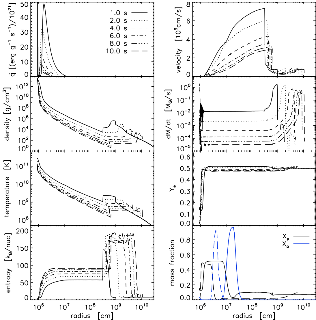
Fig. 5. Radial profiles of the net neutrino-heating rate \dot{q} , density, temperature, entropy (left, from top to bottom), velocity, mass loss rate, electron fraction Y_e , and mass fractions of free protons and \alpha particles for the neutrino wind in model M15-11-r1 at different postbounce times. For the mass fractions only the information for the first and last moments of time is provided. The wind termination shock is clearly visible in its effects on the velocity, density, temperature, and entropy of the outflow.
