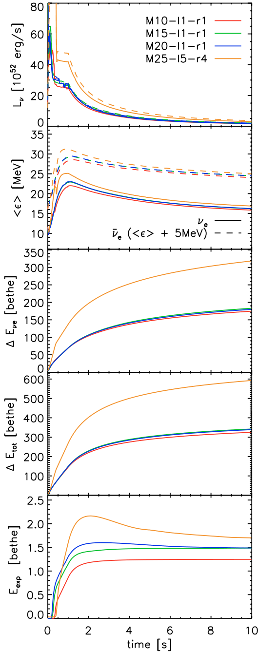
Fig. 7. For a set of simulations with different progenitor stars, M10-11-r1, M15-11-r1, M20-11-r1, and M25-15-r4, the different panels show as functions of time (from top to bottom): the radiated luminosities of \nu_e and \bar{\nu}_e , the mean energies and rms energies of these neutrinos (all measured at a distance of 500 km, disregarding gravitational redshift effects), the cumulative energy emitted in \nu_e and \bar{\nu}_e , \Delta E_{\nu_e} , the total energy released in neutrinos and antineutrinos of all flavors, \Delta E_{\text{tot}} , and the explosion energy of the models.
