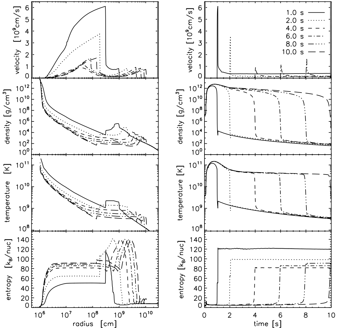
Fig. 13. Left, from top to bottom: radial profiles of the velocity, density, temperature, and entropy in model M15-1t1-r4 at different postbounce times. The profiles should be compared with the corresponding ones of model M15-1t1-r1 in Fig. 5. Right: the same quantities as functions of time for some mass shells ejected in the neutrino-driven outflow of model M15-1t1-r4. For comparison with Model M15-1t1-r1, see Fig. 6.
