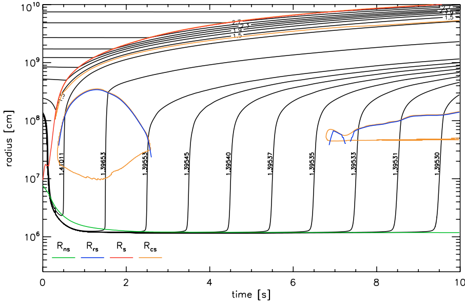
Fig. 11. Same as Fig. 3, but for model M15-lt1-r4. Here the explosion occurs at 0.22 s after bounce and because of the assumed fast subsequent decay of the neutrino luminosity, the reverse shock reveals a much different behavior than in case of model M15-l1-r1. It temporarily disappears when a subsonic breeze instead of a wind develops after about 2.5 s. At t \gtrsim 7 s the outflow expansion becomes supersonic again and a wind termination shock appears again.
