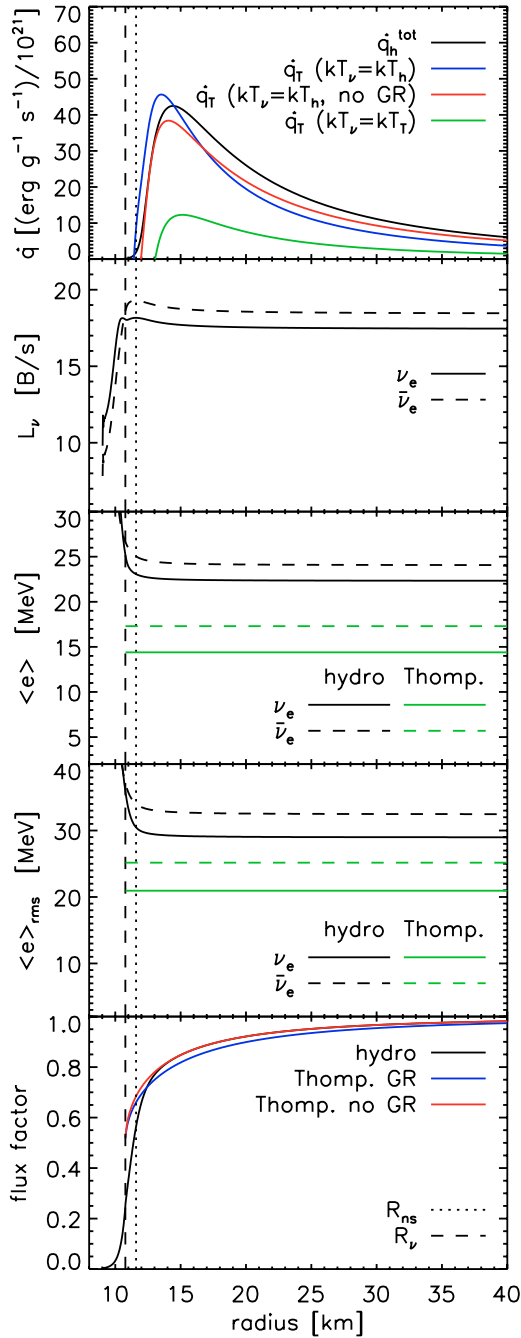
Fig. 2. Radial profiles of the net total neutrino heating rate \dot{q}^{\text{tot}} (top), \nu_e and \bar{\nu}_e luminosities L_\nu (second panel, in bethe per second or 10^{51} erg \text{s}^{-1} ), mean neutrino energies \langle \epsilon_\nu \rangle (third panel; Eq. (8)), rms energies \langle \epsilon_\nu \rangle_{\text{rms}} (fourth panel; Eq. (9)), and flux factor for model M15-11-r1 at 1.5 s after bounce. For comparison with Thompson et al. (2001), we also show \langle \epsilon_\nu \rangle and \langle \epsilon_\nu \rangle_{\text{rms}} as used in that paper, rescaled to our values of L_{\nu_e} and L_{\bar{\nu}_e} , the flux factor with and without relativistic corrections from that work, and the Newtonian and GR charged-current heating plus cooling rates using Thompson et al.’s formulas, evaluated with our neutrino luminosities and rms energies (red and blue curves) or with the rescaled rms energies of Thompson et al. (green curve). The vertical dashed line marks the position of the \nu_e -sphere, and the vertical dotted line the neutron star “surface” at a density of 10^{11} g \text{cm}^{-3} .
