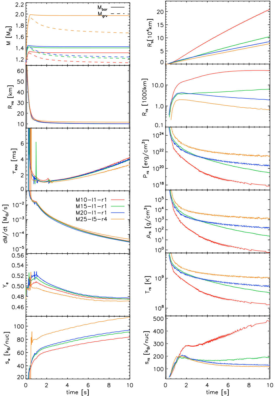
Fig. 8. Time evolution of different quantities for a set of simulations with different progenitor stars, M10-11-r1, M15-11-r1, M20-11-r1, and M25-15-r4. Shown are the baryonic mass, M_{\text{bar}} , and gravitational mass, M_{\text{grv}} (Eq. (7)), neutron star radius, neutrino-wind expansion timescale according to Eq. (15), wind mass-loss rate, electron fraction, and entropy per nucleon ( left, from top to bottom ), radius of the supernova shock, radius of the reverse shock, and pressure, density, temperature, and entropy per nucleon downstream of the reverse shock.
