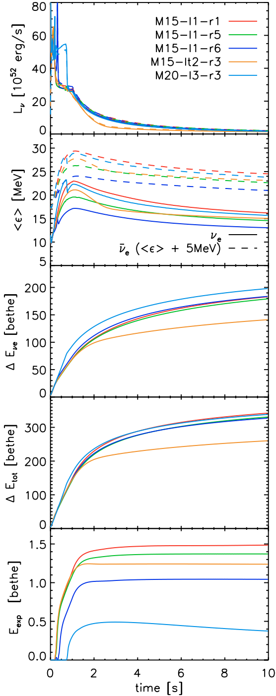
Fig. 9. The same as Fig. 7, but for simulations with varied inner boundary conditions (for clarity, however, we omitted the lines showing the rms energies of the radiated \nu_e and \bar{\nu}_e and shifted the \bar{\nu}_e energies by 5 MeV). The models M15-11-r5, M15-11-r6, M15-lt2-r3, and M20-13-r3 are compared with our reference 15 M_\odot model M15-11-r1 in order to demonstrate the influence of different neutron star radii, neutron star masses, and core neutrino luminosities at the inner grid boundary.
