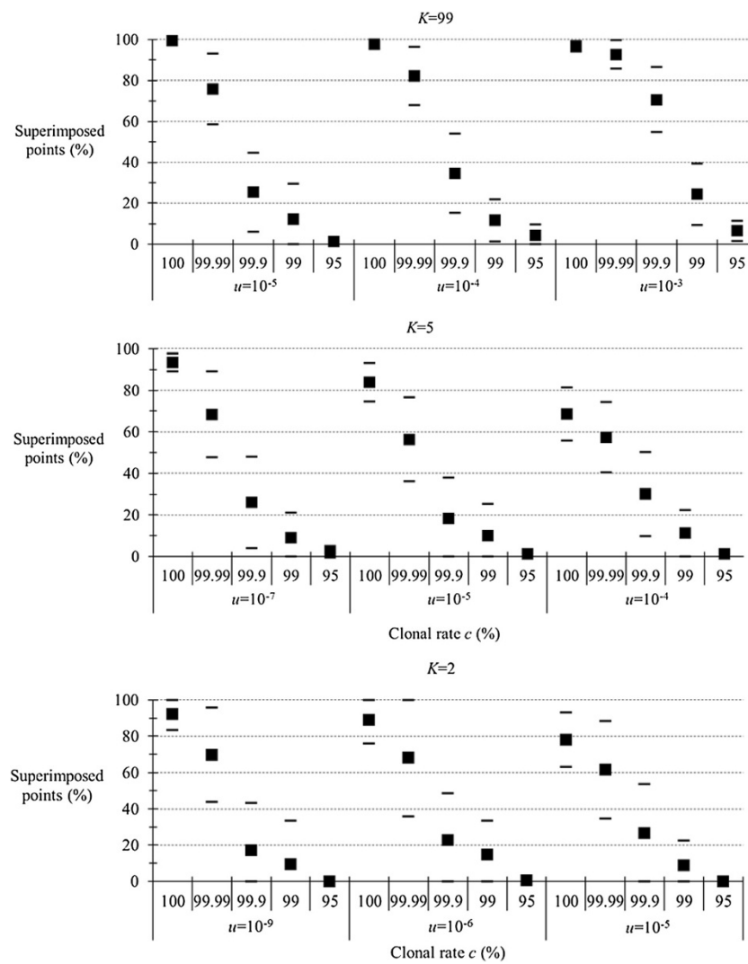
Figure 4 Proportion of superimposed points (in percent) between expected and observed F_{IS} for different levels (percent) of clonality ( c ) for different mutation rates ( u ) and different degrees of homoplasy ( K = 99, K = 5, K = 2 ) in an island model of migration.
