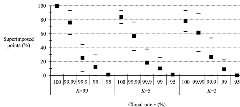
Figure 3 Proportion of superimposed points (in percent) between expected and observed F_{IS} for different levels (percent) of clonality ( c ) for different degrees of homoplasmy: low ( K = 99 ), medium ( K = 5 ) and maximum ( K = 2 ) in an island model with u = 10^{-5} and m = 0.01 .
