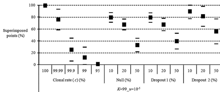
Figure 5 Proportion of superimposed points (in percent) between expected and observed F_{IS} for different levels of clonality (Clonal rate, in percent), for different proportions of allelic dropouts with model 1 and model 2 (Dropout 1 and Dropout 2) and of null alleles (Null) in an island model of migration with c = 1, K = 99, m = 0.01 and u = 10^{-5} .
