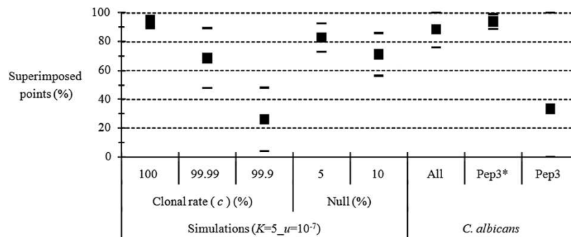
Figure 6 Proportion of superimposed points (in percent) between expected and observed F_{IS} corresponding to Candida albicans [27] as compared to the proportions of superimposed points obtained by simulations with K = 5 , u = 10^{-7} , m = 0.01 , different levels (percent) of clonality (Clonal rate) and various proportions of null alleles ("Null") in an island migration model. For the C. albicans data, analyses concerned all polymorphic loci (All), all polymorphic loci but locus Pep3 (Pep3*) and Pep3 taken alone (Pep3).
