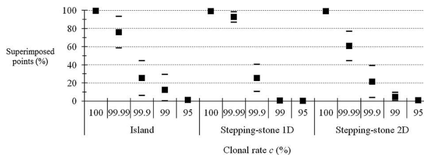
Figure 1 Proportion of superimposed points (in percent) between expected and observed F_{IS} for different levels (percent) of clonality ( c ) in different migration models: island model (Island) with m = 0.01 (migration rate), one-dimension stepping stone model (Stepping-stone 1D) with m = 0.5 , and two-dimension stepping stone model (Stepping-stone 2D) with m = 0.05 . The maximum number of alleles per locus was K = 99 and the mutation rate was \mu = 10^{-5} .
