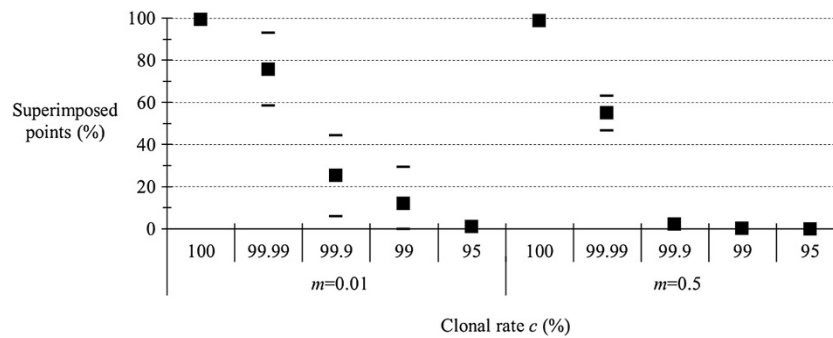
Figure 2 Proportion of superimposed points (in percent) between expected and observed F_{IS} for different levels (percent) of clonality ( c ), for different migration rates ( m ) in an island model with K = 99 and u = 10^{-5} .
