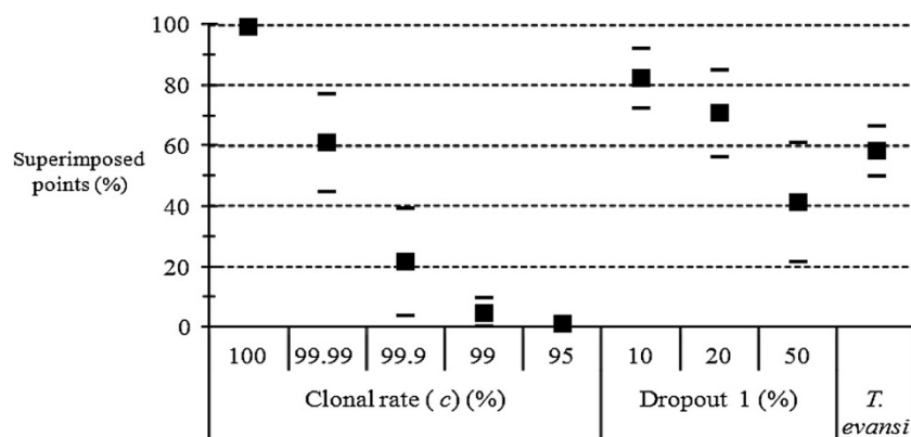
Figure 8 Proportion of superimposed points (in percent) between expected and observed F_{IS} corresponding to Trypanosoma evansi [32] compared to the proportions of superimposed points (in percent) obtained by simulations of a two-dimension stepping-stone model with K = 99 , u = 10^{-5} , m = 0.05 , various clonal rates (Clonal rate) and proportions of allelic dropouts (model 1) (Dropout 1).
