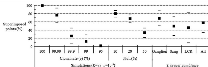
Figure 7 Proportion of superimposed points (in percent) between expected and observed F_{IS} corresponding to Trypanosoma brucei gambiense [28] compared to the proportion of superimposed points obtained by simulations with K = 99 , u = 10^{-5} , m = 0.01 , different levels of clonality (Clonal rate) and various proportions of null alleles (Nulls in%) in an island model of migration. T. brucei gambiense DNA was amplified from different fluids: lymph of cervical node (Lymph), blood (Blood) and Cerebrospinal Fluid (CSF).
