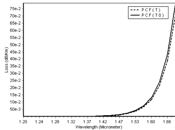
Fig. 12. Confinement loss characteristics as a function of wavelength at room temperature (solid line) and at 500^\circ\text{K} (dash line) for PCF with the following parameters; \Lambda = 1 \mu\text{m} and d_2 = 0.8 \mu\text{m} , d_1 = 0.39 \mu\text{m} and N=6
