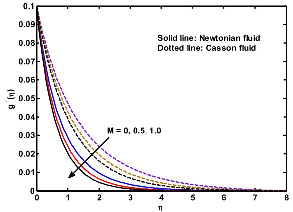
Fig. 3. Influence of M on g'(\eta) .
