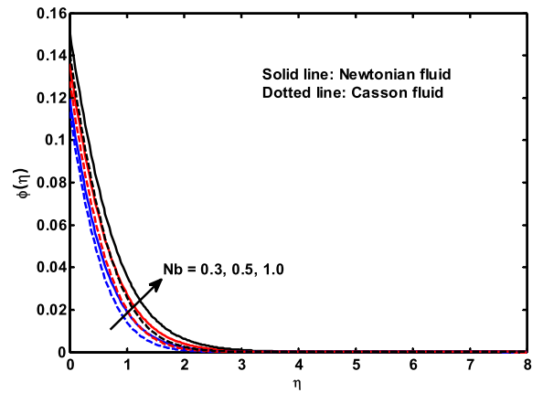
Fig. 18. Influence of Nb on \phi(\eta) .
