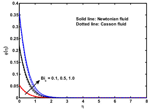
Fig. 17. Influence of Bi_c on \phi(\eta) .
