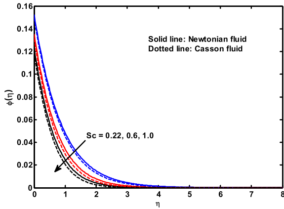
Fig. 15. Influence of Sc on \phi(\eta) .
