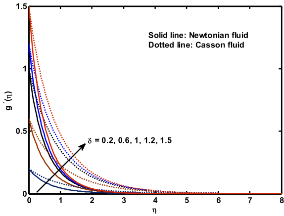
Fig. 5. Influence of \delta on g'(\eta) .
