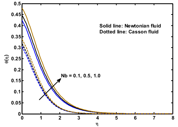
Fig. 9. Influence of Nb on \theta(\eta) .
