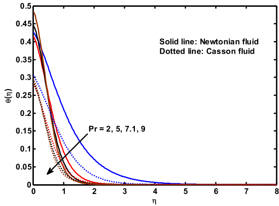
Fig. 6. Influence of Pr on \theta(\eta) .
