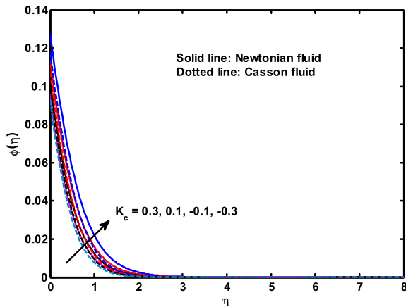
Fig. 16. Influence of Kc on \phi(\eta) .
