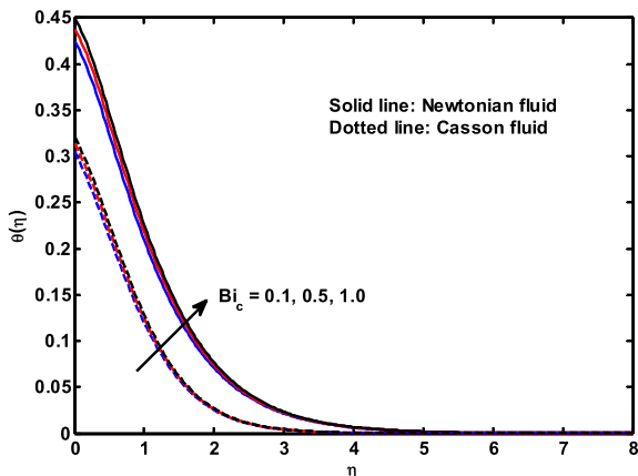
Fig. 13. Influence of Bi_c on \theta(\eta) .
