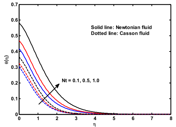
Fig. 10. Influence of Nt on \theta(\eta) .
