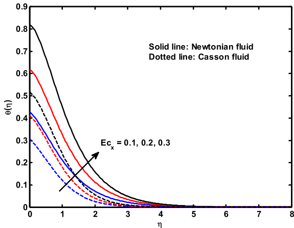
Fig. 11. Influence of Ec_x on \theta(\eta) .
