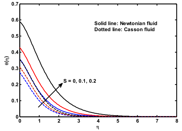
Fig. 8. Influence of S on \theta(\eta) .
