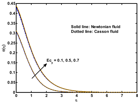
Fig. 12. Influence of Ec_y on \theta(\eta) .
