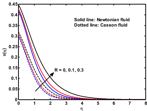
Fig. 7. Influence of R on \theta(\eta) .
