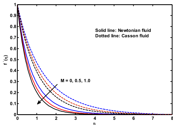
Fig. 2. Influence of M on f'(\eta) .
