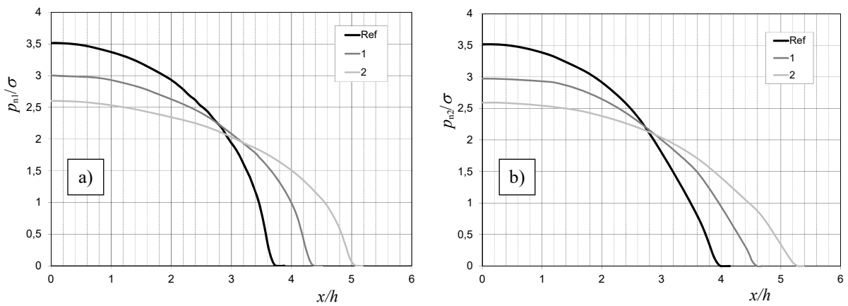
Fig. B7 Contact pressure distributions for different material properties of the indenter for R/h = 500 ; a) at the indenter-layer interface, b) at the layer-substrate interface
