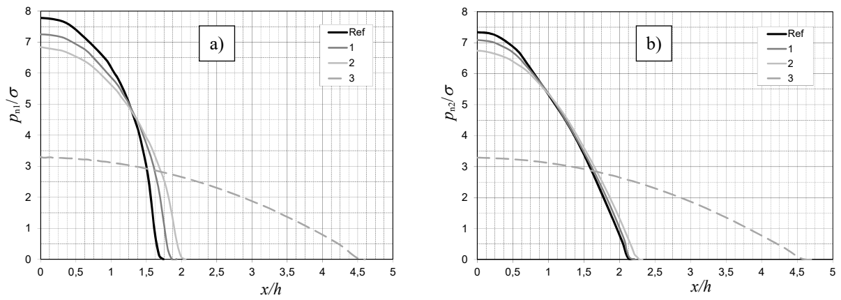
Fig. B2 Contact pressure distributions for different material properties of the layer for R/h = 100 ; a) at the indenter-layer interface, b) at the layer-substrate interface
