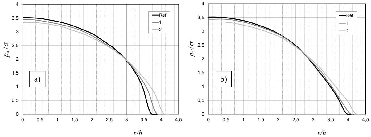
Fig. B8 Contact pressure distributions for different material properties of the layer for R/h = 500 ; a) at the indenter-layer interface, b) at the layer-substrate interface
