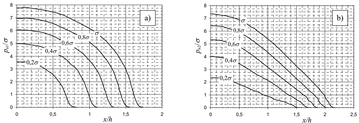
Fig. A1 Contact stresses for different load intensities for R/h = 100 : a) indenter-layer interface, b) layer-substrate interface
