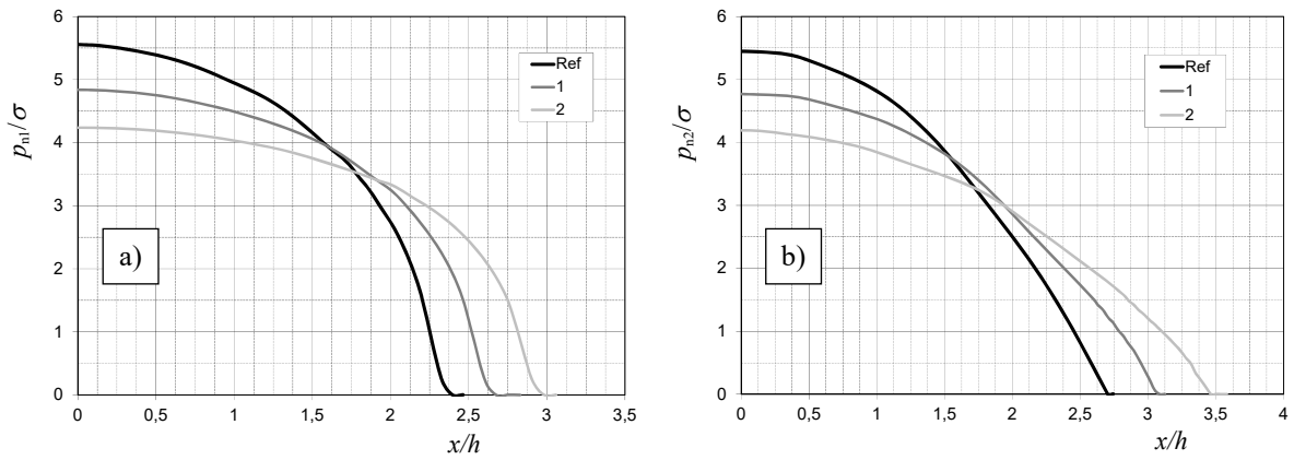
Fig. B6 Contact pressure distributions for different material properties of the substrate for R/h = 200 ; a) at the indenter-layer interface, b) at the layer-substrate interface
