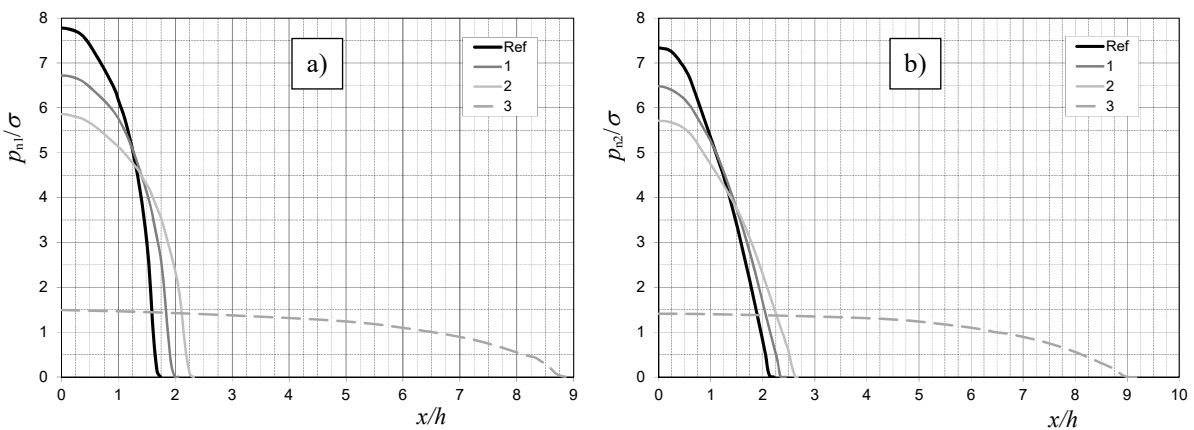
Fig. B1 Contact pressure distributions for different material properties of the indenter for R/h = 100 : a) at the indenter-layer interface, b) at the layer-substrate interface
