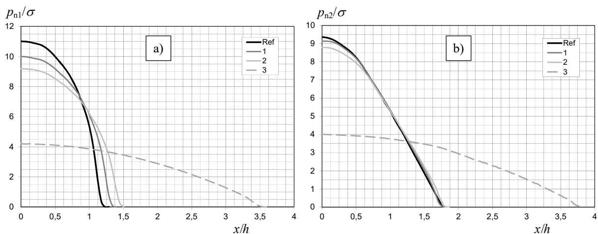
Fig. 10 Contact pressure distributions for different material properties of the layer; a) at the indenter-layer interface, b) at the layer-substrate interface
