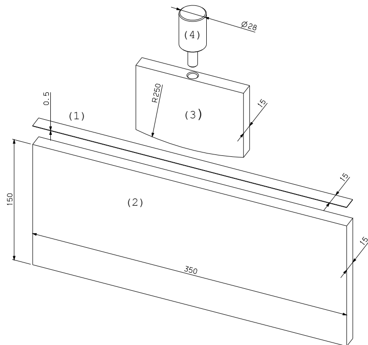
Fig. 12 Experimental model: (1) layer, (2) substrate, (3) cylindrical indenter, (4) shoulder for the grip of the testing machine
