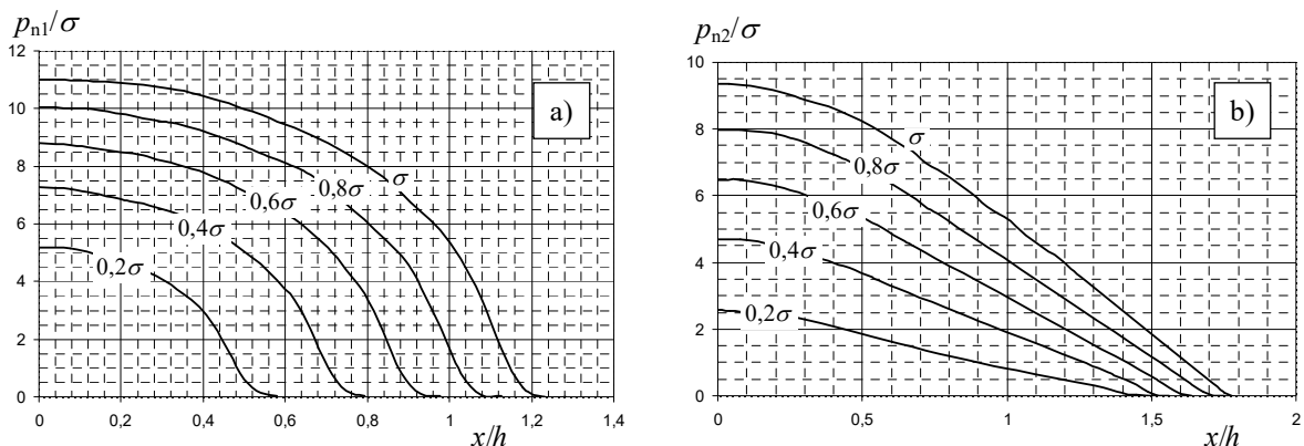
Fig. 5 Contact stresses for different load intensities: a) indenter-layer interface, b) layer-substrate interface
