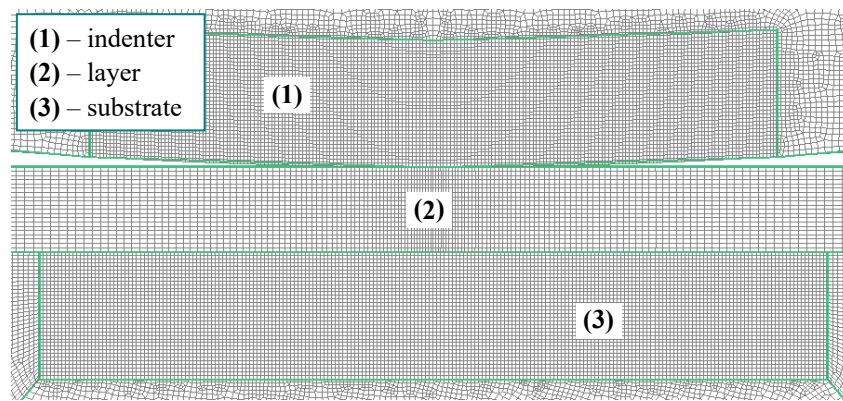
Fig. 2 Mesh detail around the initial point of contact
