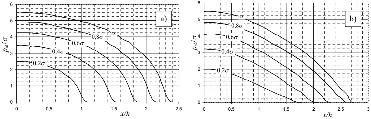
Fig. A2 Contact stresses for different load intensities for R/h = 200 : a) indenter-layer interface, b) layer-substrate interface
