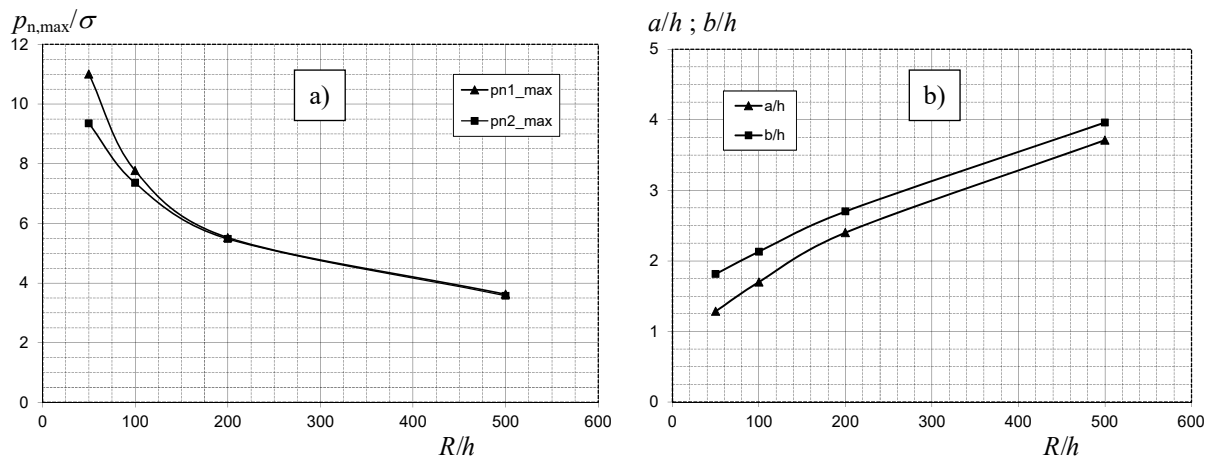
Fig. 8 Values of (a) maximal contact pressures and (b) contact half-widths with respect to R/h at full load
