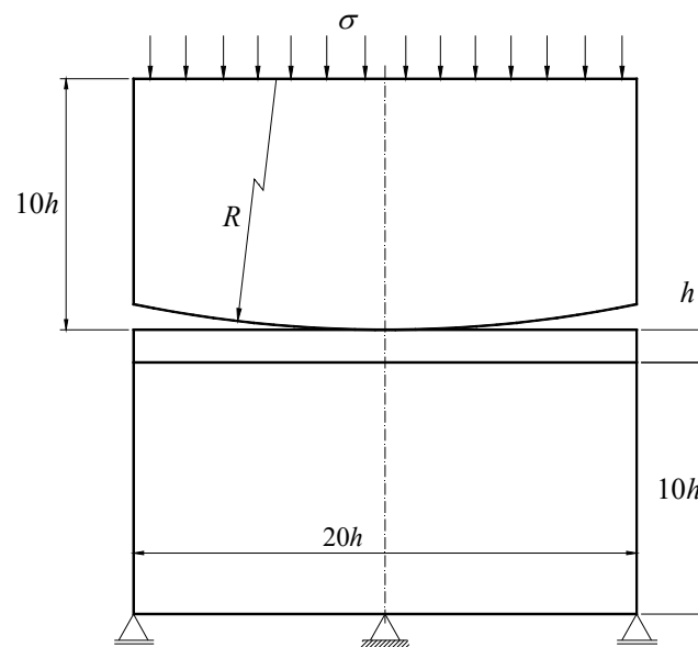
Fig. 1 Geometry of the FEM model
