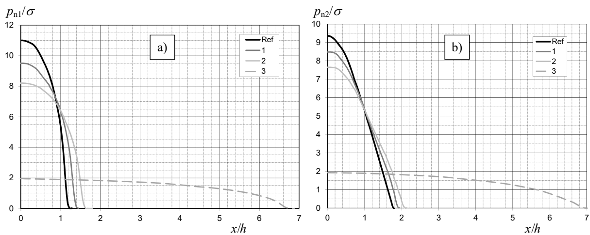
Fig. 9 Contact pressure distributions for different material properties of the indenter; a) at the indenter-layer interface, b) at the layer-substrate interface
