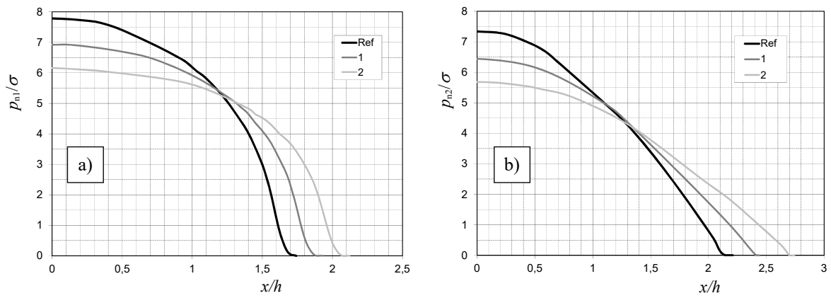
Fig. B3 Contact pressure distributions for different material properties of the substrate for R/h = 100 ; a) at the indenter-layer interface, b) at the layer-substrate interface
