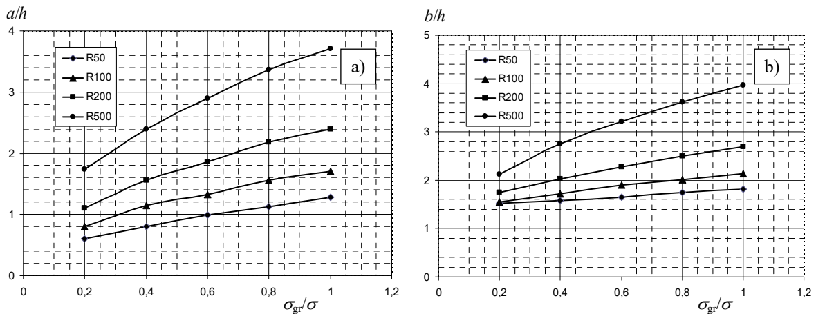
Fig. 7 Variation of contact half-width with load intensity for all R/h geometries; a) at the indenter-layer interface, b) at the layer-substrate interface
