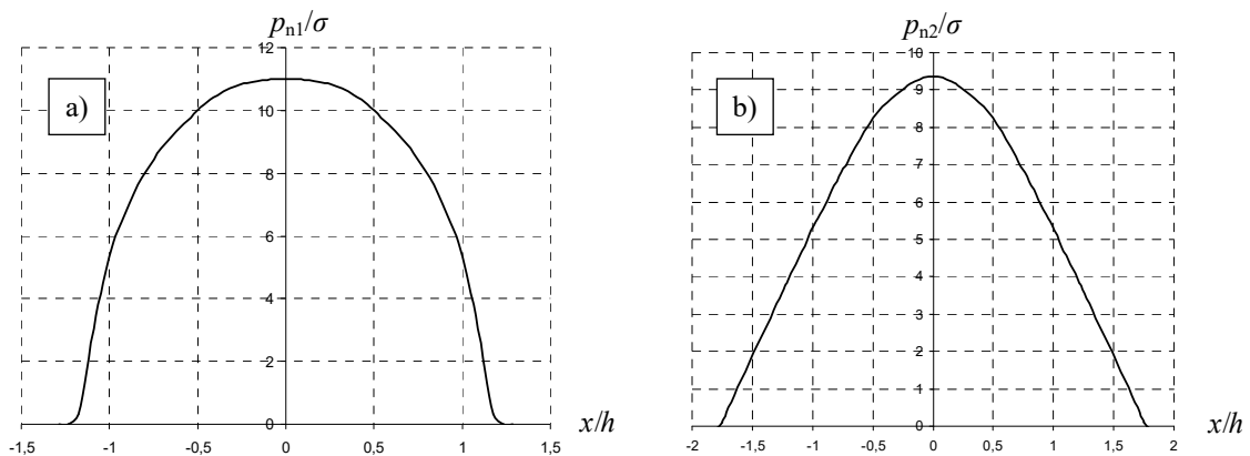
Fig. 4 Contact pressure distributions for the initial geometry R/h = 50 : a) at the indenter-layer interface p_{n1,max} / \sigma \approx 11 ; a/h \approx 1.29 ; b) at the layer-substrate interface p_{n2,max} / \sigma \approx 9.35 ; b/h \approx 1.78
