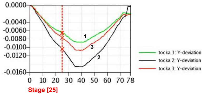
Fig. 14 Measured vertical displacements ( y direction) of three reference points; e.g. at stage 25 (after 25 s) the force equals approximately 1070 N
