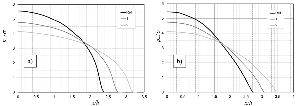
Fig. B4 Contact pressure distributions for different material properties of the indenter for R/h = 200 ; a) at the indenter-layer interface, b) at the layer-substrate interface
