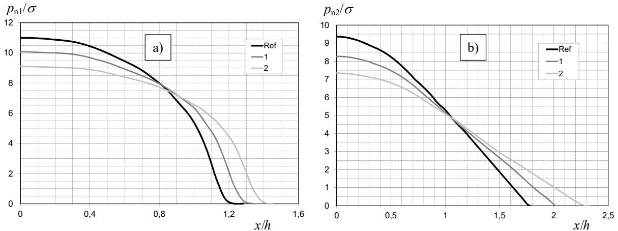
Fig. 11 Contact pressure distributions for different material properties of the substrate; a) at the indenter-layer interface, b) at the layer-substrate interface
