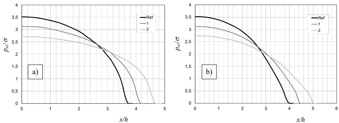
Fig. B9 Contact pressure distributions for different material properties of the substrate for R/h = 500 ; a) at the indenter-layer interface, b) at the layer-substrate interface
