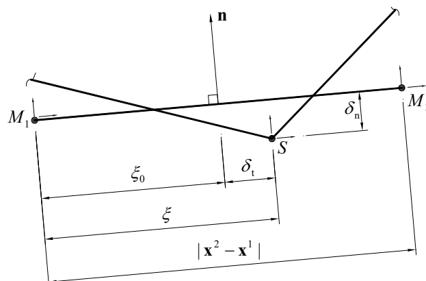
Fig. 3 Three-node slide line element: \xi, \xi_0 – current and previous surface coordinate, \delta_n – penetration of slave node into the master segment, \delta_t – sliding of the slave node on the master segment
