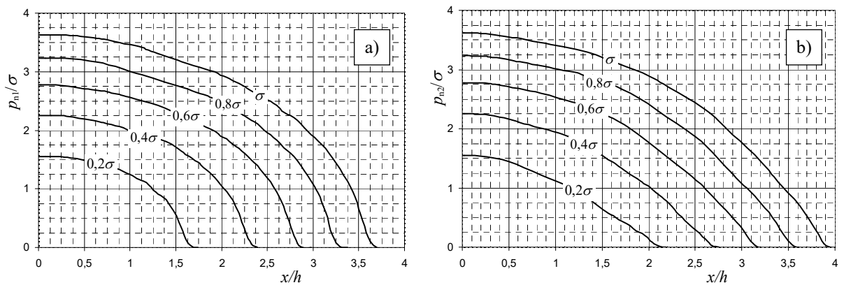
Fig. A3 Contact stresses for different load intensities for R/h = 500 : a) indenter-layer interface, b) layer-substrate interface
