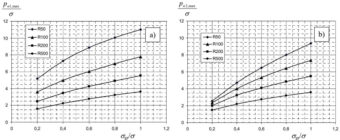
Fig. 6 Variation of maximal contact pressures with load intensity for all R/h geometries; a) at the indenter-layer interface, b) at the layer-substrate interface
