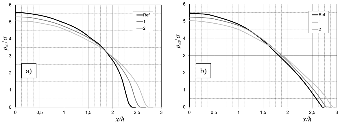
Fig. B5 Contact pressure distributions for different material properties of the layer for R/h = 200 ; a) at the indenter-layer interface, b) at the layer-substrate interface
