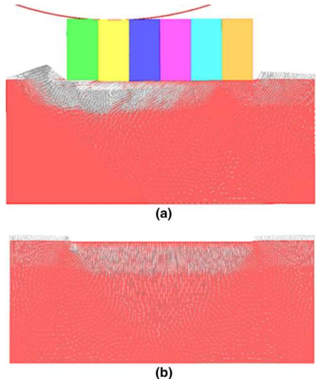
Fig. 25—Displacement vectors during (a) incremental-forming and (b) conventional-forging process.
