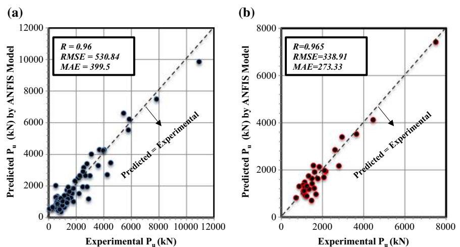
Fig. 3 Predicted versus experimental P_u values using the optimal ANFIS model: a training (learning and validation) datasets, b testing datasets
