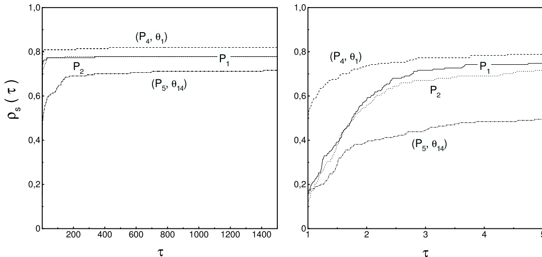
Figure 1: Comparison of methods P_1 , P_2 , (P_4, \theta_1) , and (P_5, \theta_{14}) using performance profiles.
