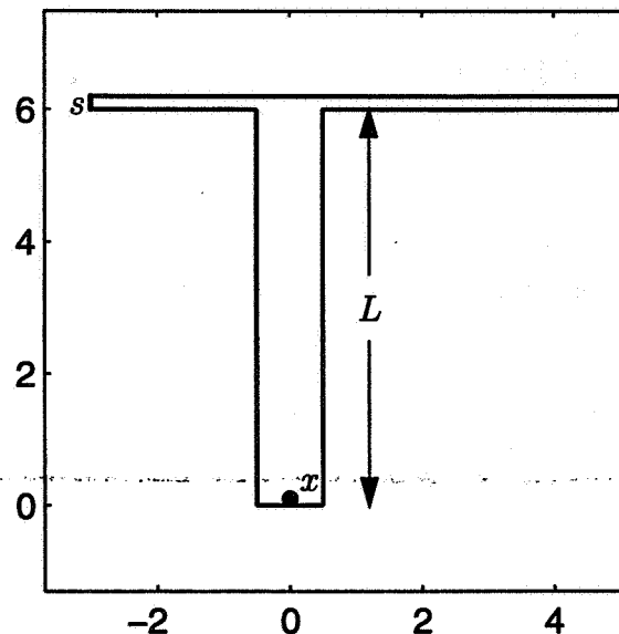
Figure 11: The BVP of Section 8 is solved on this T-shaped region. The length L is allowed to vary, and the forced edge is denoted s . The point x at which the solution is sought is at 0.1i . The dimensions of the horizontal bar are 8 \times 0.2 .
