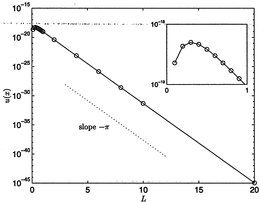
Figure 12: Solution of the BVP for the region in Fig. 11. The inset shows the solution at points for L < 1 . As L grows, the curve quickly approaches k \cdot e^{-\pi L} , corresponding to the leading-order behavior of the solution for a rectangle.
