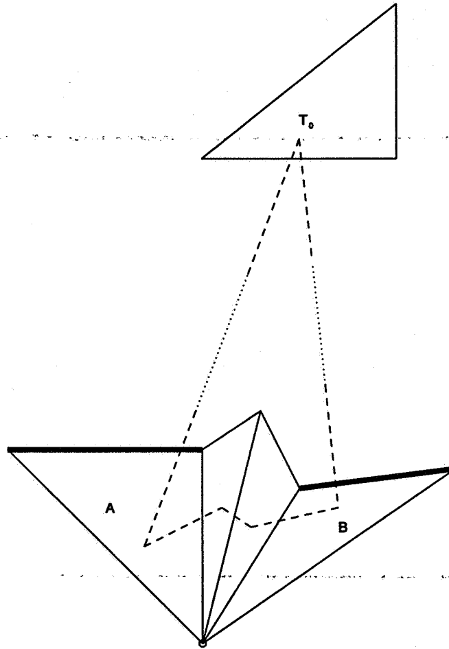
Figure 4: An illustration of the contradiction that would arise if two different triangles in the triangulation had the same new vertex. If triangles A and B , whose entry diagonals are shown as heavy lines, both shared this new vertex (marked by the circle), there would be a cycle in the dual graph (marked by dashed lines).
