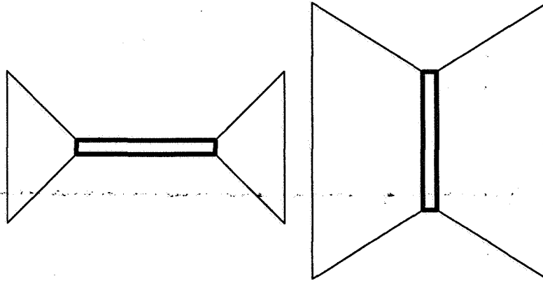
Figure 2: On the left is an octagon with a long, narrow quadrilateral in its triangulation (heavy outline). This quadrilateral would have to have its sides split because of crowding: in a mapping with conformal center at the center of the quadrilateral, the short edges of the quadrilateral are exponentially contracted in the preimage on the disk. In contrast, for the polygon on the right no splitting is necessary, because the polygon is “fat” around the quadrilateral. That is, the quadrilateral can be enclosed in a disk that is mostly interior to the polygon.
