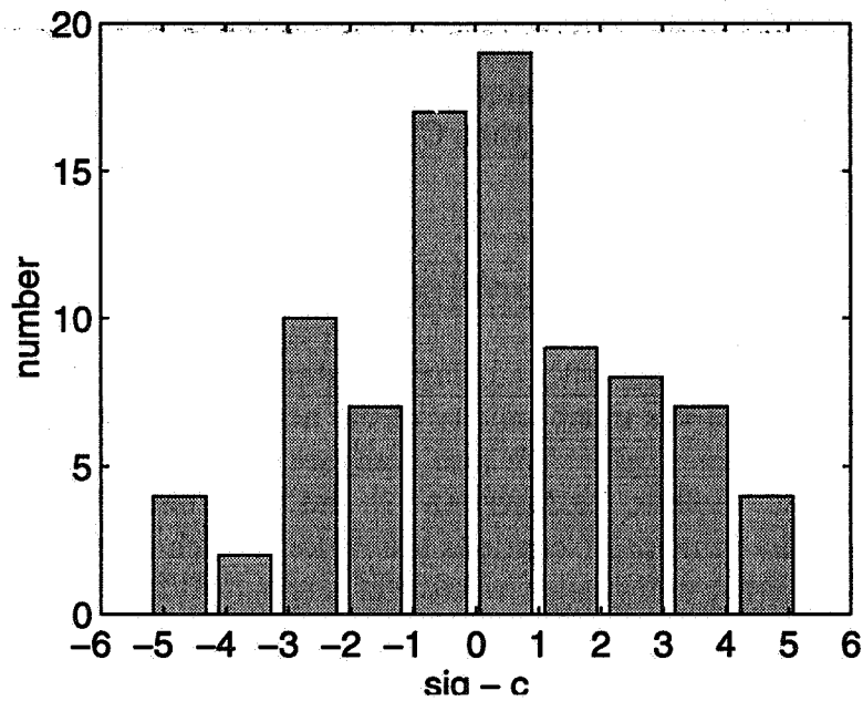
Figure 6: Evidence of controlled cross-ratio sizes. The histogram depicts the discrepancies \sigma_i - c_i between the primitive cross-ratio variables and polygon cross-ratios for the experiments in Section 7. The variables are logarithmic. The clustering near zero and absence of large outliers supports the claim that CRDT circumvents crowding.
