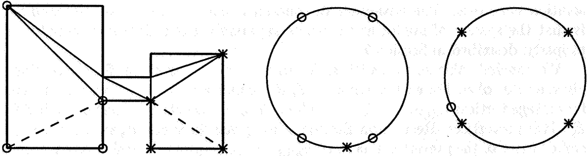
Figure 5: On the left is a triangulated polygon with two distinguished quadrilaterals whose diagonals are given as dashed lines: No embedding of the S-C prevertices will be universally uncrowded. In the middle picture we see an embedding that keeps the prevertices of the first quadrilateral (marked with circles) uncrowded, while the prevertices of the other (marked with stars) are crowded—too closely to be distinguished. However, in another embedding (far right), the crowding situation is reversed.
