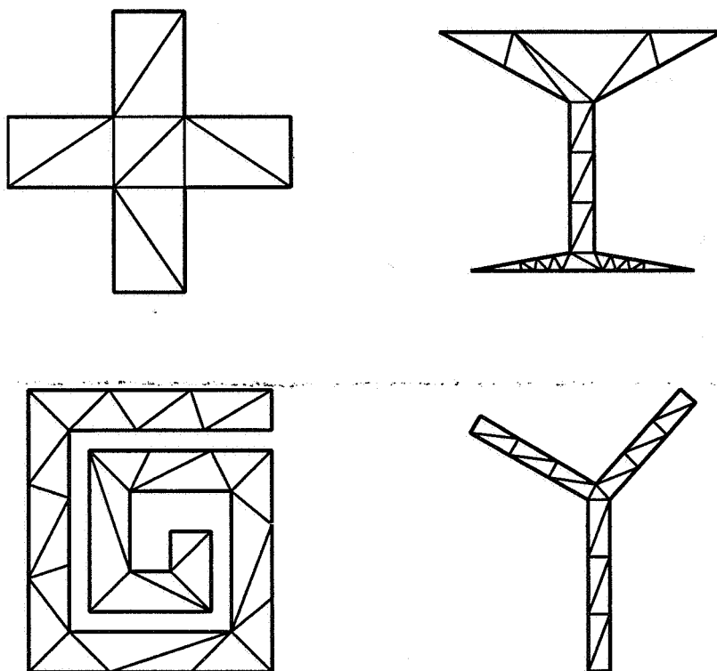
Figure 9: Four regions on which CRDT experiments were performed, after splitting and Delaunay triangulation. See text.
