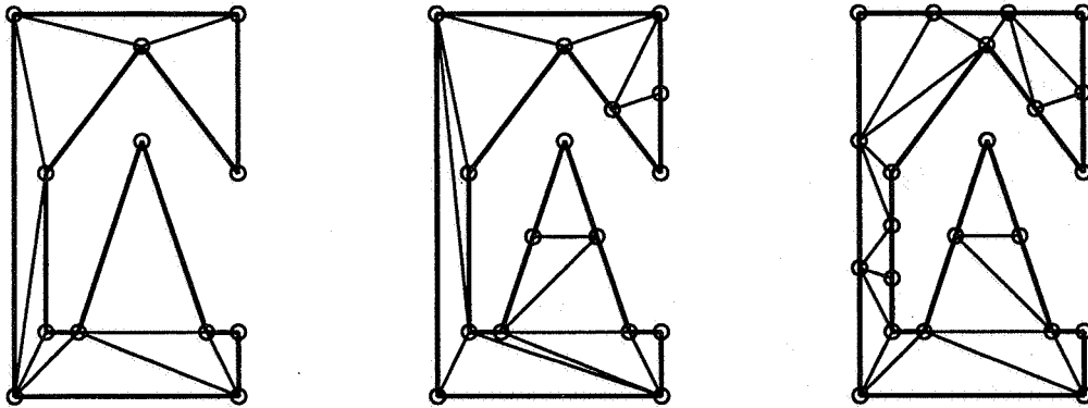
Figure 3: On the left is the Delaunay triangulation of a polygon. The middle shows the Delaunay triangulation after the sharp corners have been chopped in the first splitting phase. On the right is the subsequent result of the second phase, in which narrow regions are subdivided and the Delaunay triangulation is recomputed.
