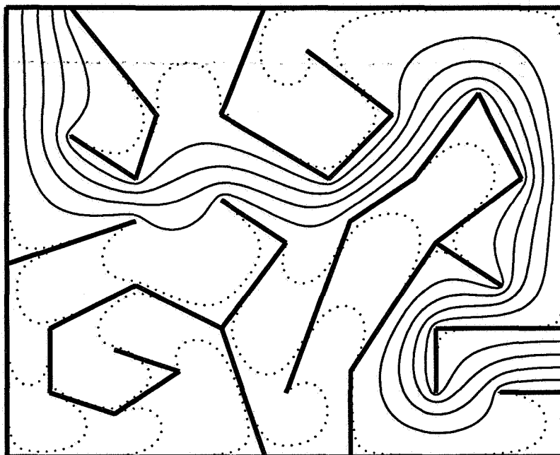
Figure 10: Rectangle map to a “maze.” The exits of the maze map to the short rectangle sides, which are normalized to unit length. The maze has several branches that are very crowded on the long rectangle sides. The solid curves in the maze are images of lines with abscissae 0.2, 0.4, 0.6, and 0.8. The preimages of the dotted curves are separated from the long rectangle edges by 10^{-2} , 10^{-4} , ..., 10^{-16} . All computations were performed in double precision.
