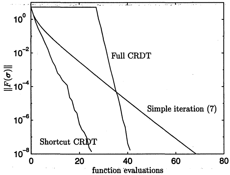
Figure 8: Convergence curves for numerical solutions of F(\sigma) = 0 . The iteration (7) converges linearly. The NESOLVE variations exhibit approximately linear convergence as well, but at much better rates.
