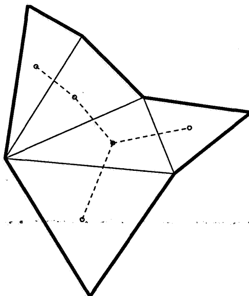
Figure 1: The Delaunay triangulation of a 7-sided polygon. The heavy solid segments are boundary edges, and the light solid segments are diagonals of the triangulation. The dual graph has five nodes (circles) and four edges (dashed lines). The dual is abstract; the geometry shown here is for convenience.
