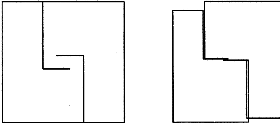
Figure 7: Lack of global convergence in the SC Toolbox. In solving for the polygon on the left, dparam arrives at the polygon on the right and terminates due to a nearby local minimum. The horizontal slits cannot move past each other without temporarily increasing the solution residual.
