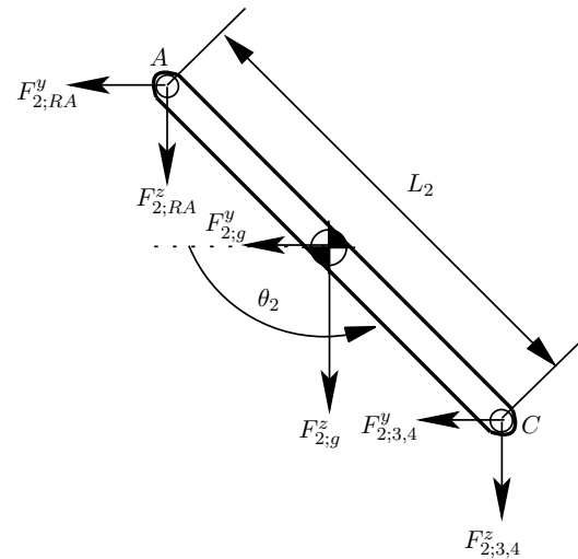
Fig. 4: Free-body diagram of link \mathcal{L}_2 in local co-ordinates.
