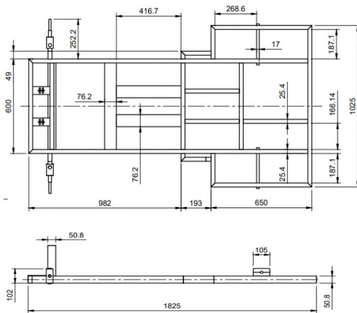
Figure 5: Design of SEM urban vehicle frames
