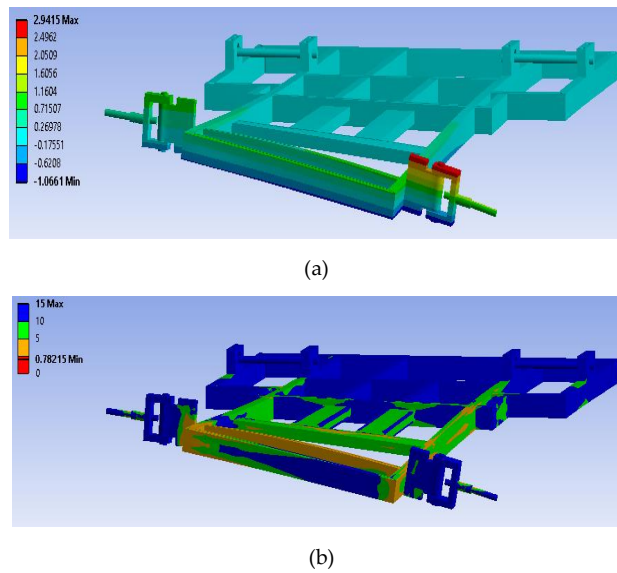
Figure 20: Deformation (a) and safety factor (b) of the ninth variation of chassis simulation
