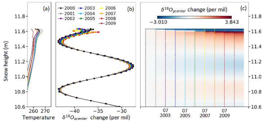
Figure 3. Simulation 2: attenuation of the seasonal \delta^{18}\text{O}_{\text{center}} variation caused by diffusion in the vapor phase over 10 years (with temperature evolution, original signal with a mean value of -35.5\text{‰} and amplitude of 16\text{‰} ). (a) Vertical temperature profile for each summer; (b) \delta^{18}\text{O}_{\text{center}} profile for each summer; (c) evolution of the deviation to the original profile of \delta^{18}\text{O}_{\text{center}} . Note that temperature evolves during the whole year (see Fig. S1).
