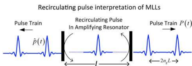
Fig. 1. Schematic of a recirculating pulse within a resonator. Mode locking in a laser has occurred when the output has periodicity of the resonator round-trip time. n_g is the group index, L is the length of the resonator. The temporal period of the pulse train is 2n_g L/c , where c is the speed of light.
