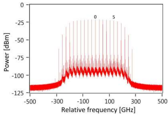
Fig. 9. Full spectrum of the MLL after the single-sideband feed-forward phase noise reduction scheme. Note that only the lower-frequency sidebands, the sidebands that possess the reduced phase noise remain in the spectrum. The original MLL and upper-frequency sidebands are suppressed by the modulation technique and no extra optical filtering is required to obtain this spectrum. Detailed quantification of the spectral quality is given in subsequent figures.
