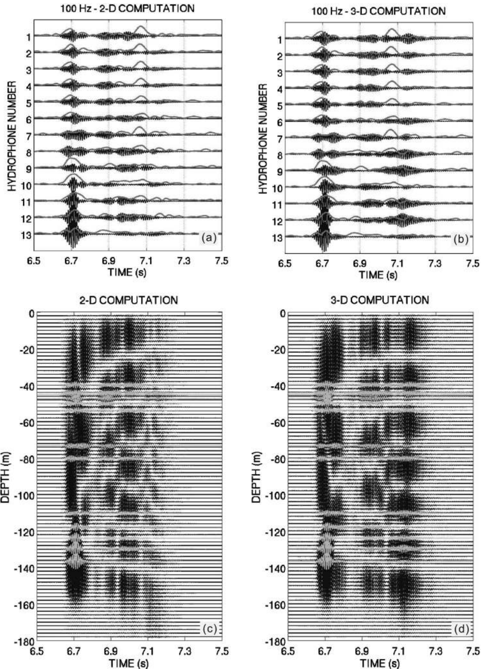
Fig. 2. Simulated time series versus hydrophone number obtained using 2D (a) and 3D (b) PE computations with 3DWAPE. The gray traces show the envelopes of the corresponding experimental data. Simulated time series versus depth obtained using 2D (c) and 3D (d) PE computations with 3DWAPE. The gray traces correspond to the simulated signals received on the 13 hydrophones.
