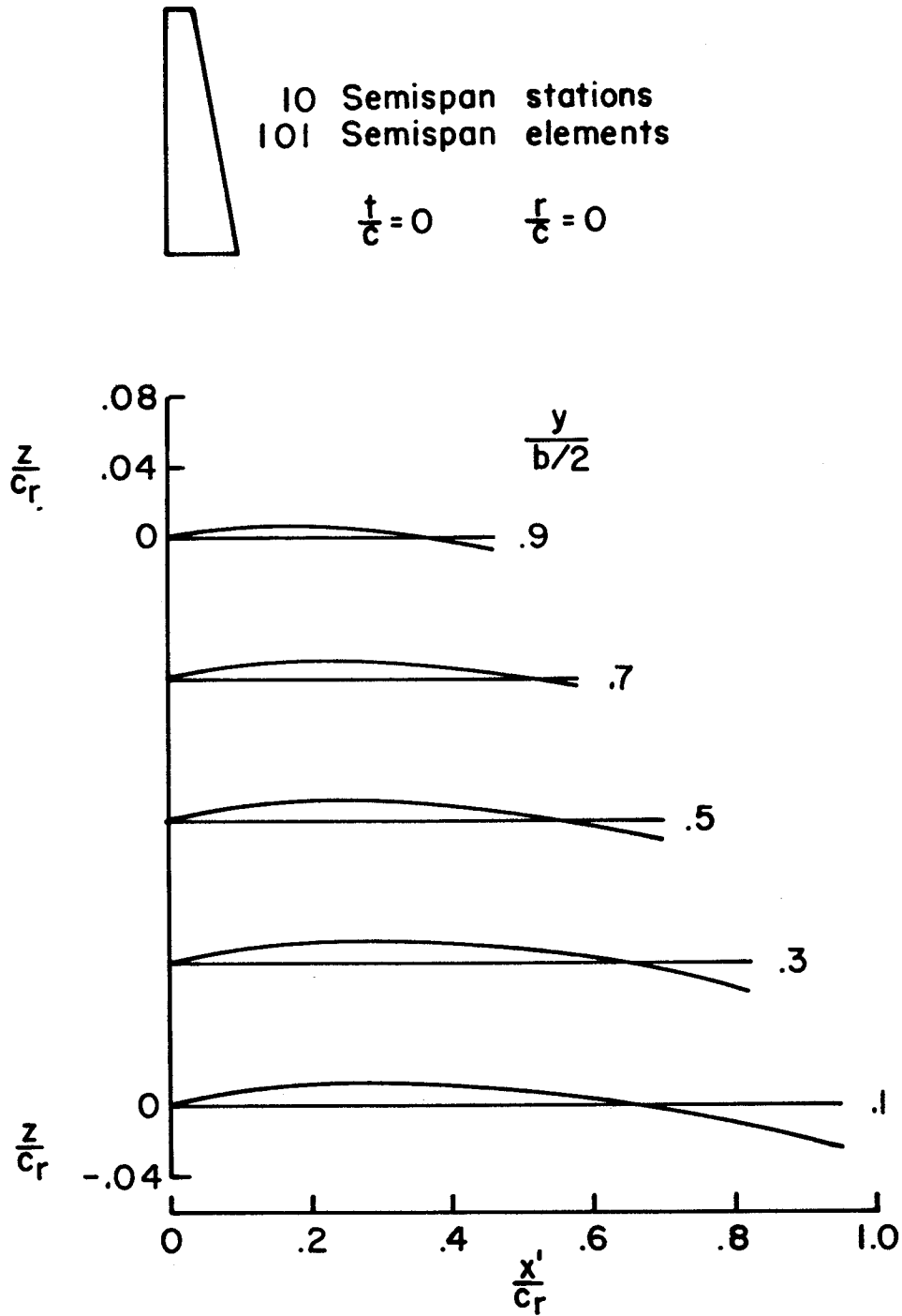
Figure 16.- Program geometric data for a general aviation wing camber surface design. M = 0.5 , R = 0.0 , C_{L,des} = 0.35 , no C_m restraint.
