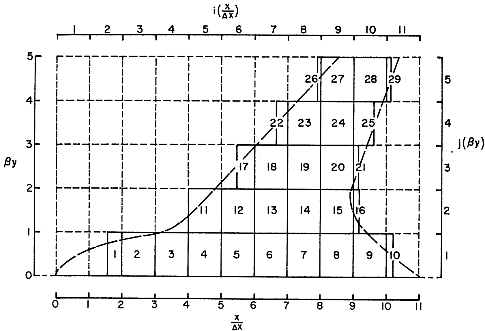
Figure 2.- Grid system used in supersonic analysis.
