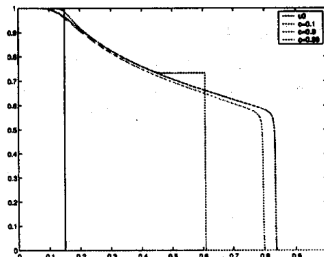
Figure 12: The numerical solutions of the Buckley-Leverett equation in non-conservative form obtained from the monotone Lax-Friedrichs scheme (13). The approximations are computed to t = 0.1 on [0, 1] with 2,500 grid points.
