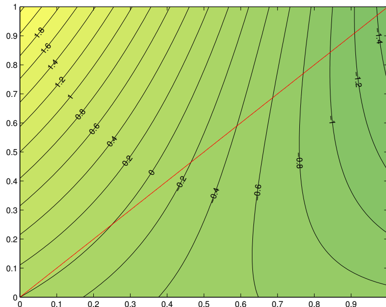
Figure 1: Active-set QP method gives uphill step
