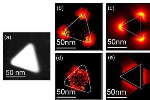
Figure 9 EELS maps of individual nanoprisms measured experimentally and compared to BEM calculations. (a) High-angle annular dark field image of a nanoprism. (b) Experimental EELS map of a dipolar mode. (c) Corresponding BEM calculation. (d) Experimental EELS map of a higher order mode. (e) Corresponding BEM calculation. Adapted from Ref. [49] with permission. Copyright (2015) American Chemical Society.
