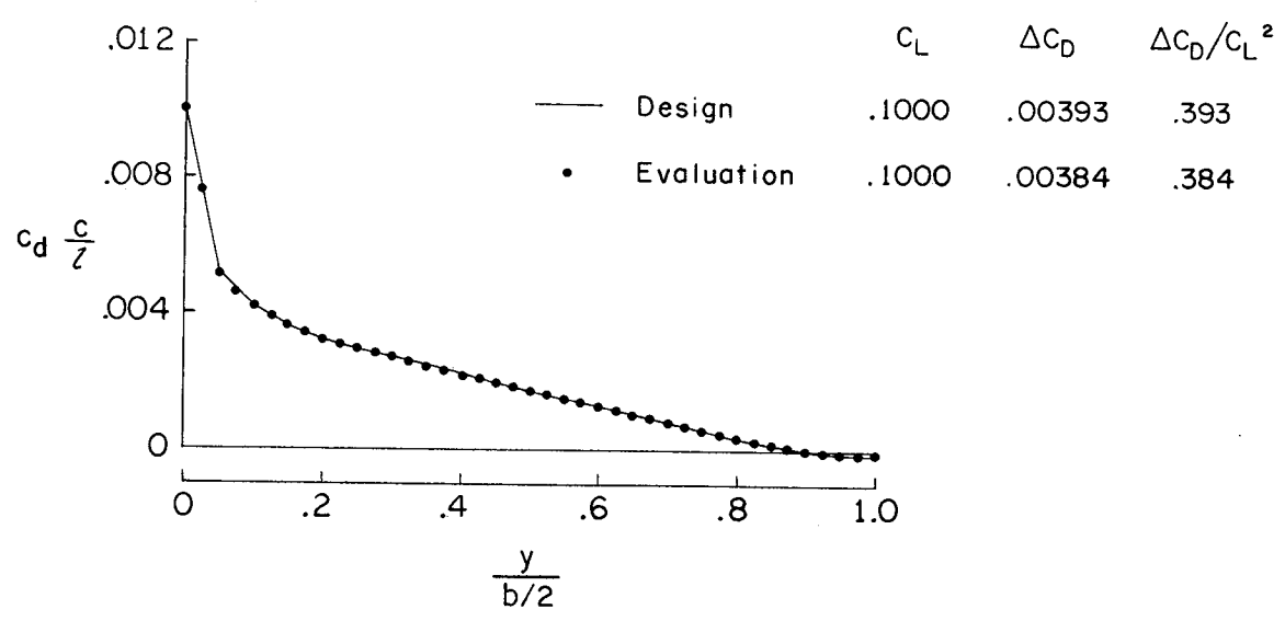
(a) Delta wing; three loadings; M = 2.0 .
