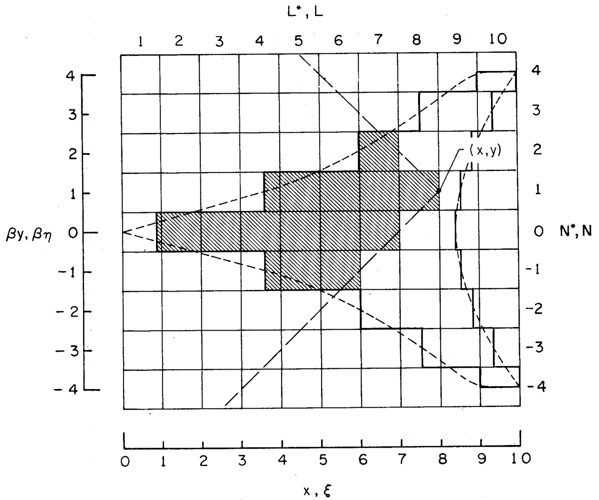
Figure 4.- Grid system used in numerical solution.
