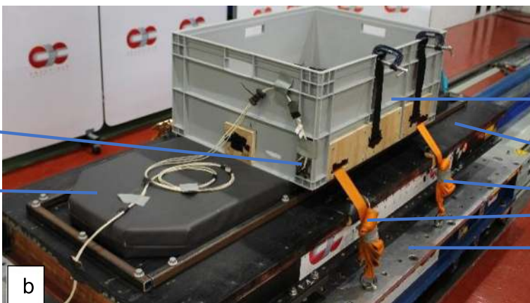
Fig. 1 a A 10-g pulse, velocity and displacement read by the sled with BS EN 1789 guidelines and b experimental setup
