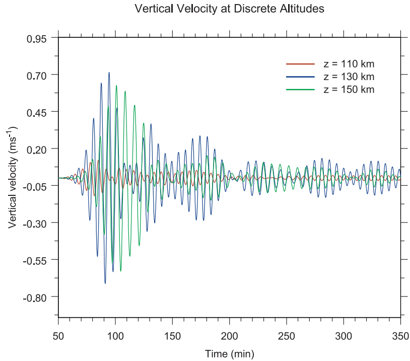
Figure 4. The vertical velocities at discrete altitudes of 110, 130, and 150 km.
