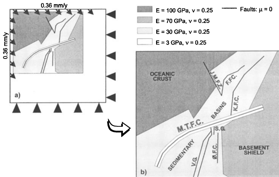
Figure 4. Geometry and mechanical parameters used for the UDEC modeling. See key in Figure 1. E = Young's modulus, \nu = Poisson's ratio, \mu = faults friction.
