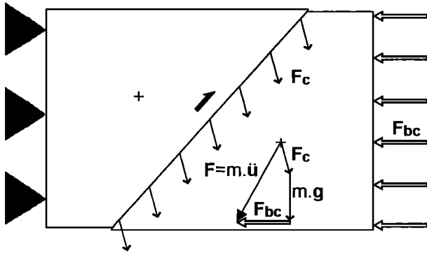
Figure A1. Distinct element method: example of out of balance forces applied to the centre of gravity of one block. F_{bc} , force arising from boundaries conditions; F_c , contact force; m \cdot g , gravitational force; F , vectorial sum of forces; m , block mass; \ddot{u} , acceleration of the center of gravity of the block.
