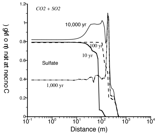
(a) Sulfate
