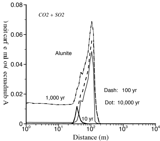
(b) Alunite
