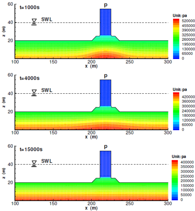
Fig. 7 The distribution of pore pressure in seabed foundation at different times in consolidation process
