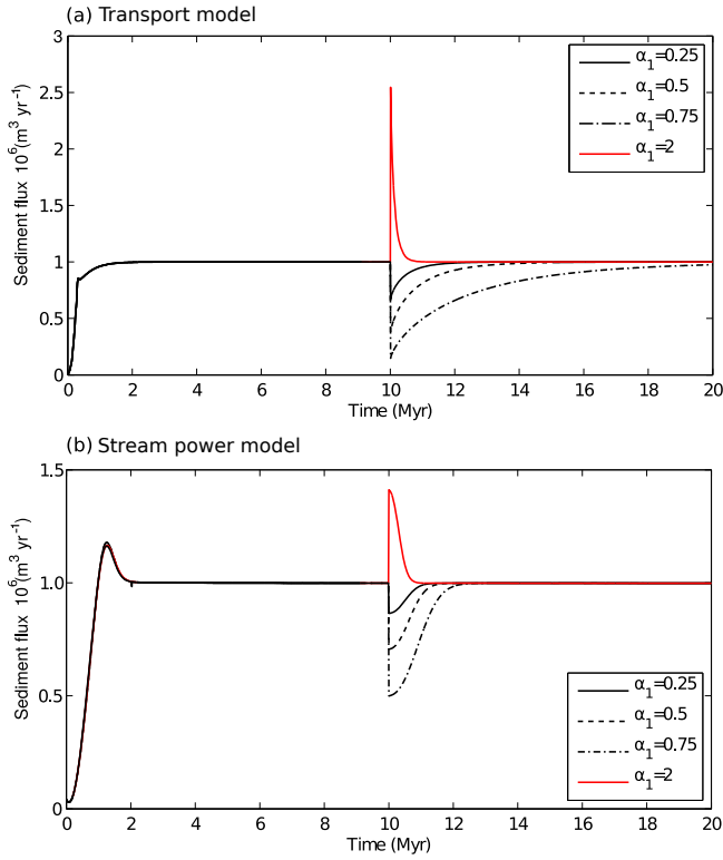
Figure 9. (a) Response of the transport model to a change in precipitation rate. Equation (6) is solved for \delta = 1.5 and c = 1 \times 10^{-4} (\text{m}^2 \text{ yr}^{-1})^{1-\delta} . The precipitation rate is initially \alpha_0 = 1 \text{ m yr}^{-1} and changes to \alpha_1 = 0.25, 0.5, 0.75 , or 2 \text{ m yr}^{-1} after 10 Myr. (b) Response of the stream power model to a change in precipitation rate. Equation (6) is solved for m = 0.5 and k = 1 \times 10^{-5} \text{ m}^{-1} (\text{m}^2 \text{ yr}^{-1})^{1-m} . The precipitation rate is initially \alpha_0 = 1 \text{ m yr}^{-1} and changes to \alpha_1 = 0.25, 0.5, 0.75 , or 2 \text{ m yr}^{-1} after 10 Myr.
