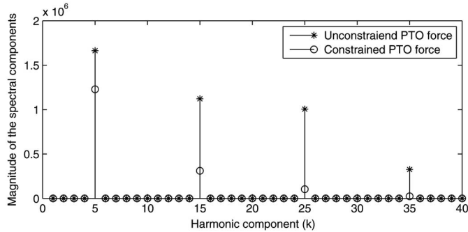
Fig. 6. Spectral components of the PTO force.
