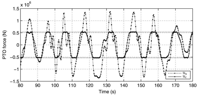
Fig. 10. Unconstrained PTO force u_u and constrained PTO force u_c for a Bretschneider sea state of T_p = 10 s and H_s = 1 m.
