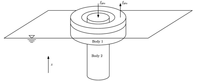
Fig. 2. Self-reacting and two-body heaving WEC.
