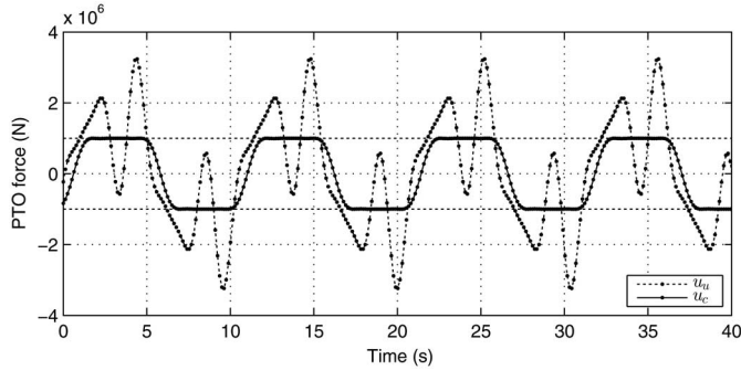
Fig. 5. Unconstrained PTO force u_u and constrained PTO force u_c for an incident regular wave of period T_w = 10 s and amplitude A = 5 m.
