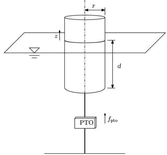
Fig. 1. Single-body heaving WEC.
