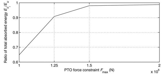
Fig. 7. Total absorbed energy as a function of the force constraint.
