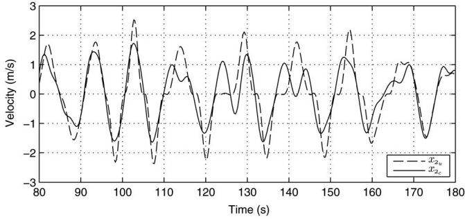
Fig. 9. Vertical velocity for a Bretschneider sea state of T_p = 10 s and H_s = 1 m: x_{2u} is the vertical velocity when the PTO force is not constrained; x_{2c} is the vertical velocity when the PTO force is constrained.
