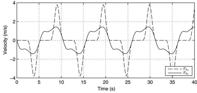
Fig. 4. Vertical velocity for an incident regular wave of period T_w = 10 s and amplitude A = 5 m: x_{2_u} is the vertical velocity when the PTO force is not constrained; x_{2_c} is the vertical velocity when the PTO force is constrained.
