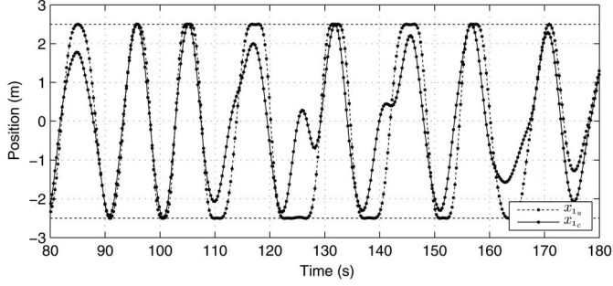
Fig. 8. Vertical position for a Bretschneider sea state of T_p = 10 s and H_s = 1 m: x_{1u} is the vertical position when the PTO force is not constrained; x_{1c} is the vertical position when the PTO force is constrained.
