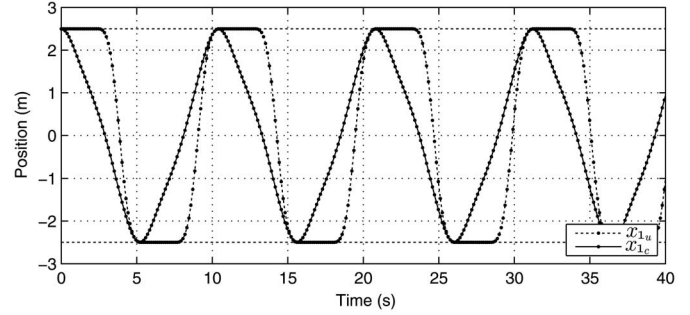
Fig. 3. Vertical position for an incident regular wave of period T_w = 10 s and amplitude A = 5 m: x_{1u} is the vertical position when the PTO force is not constrained; x_{1c} is the vertical position when the PTO force is constrained.
