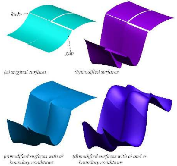
Fig. 15. Modification of a set of 4 surfaces.
