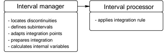
Fig. 3. Schematic of adaptive through-thickness integration algorithm for shell elements.
