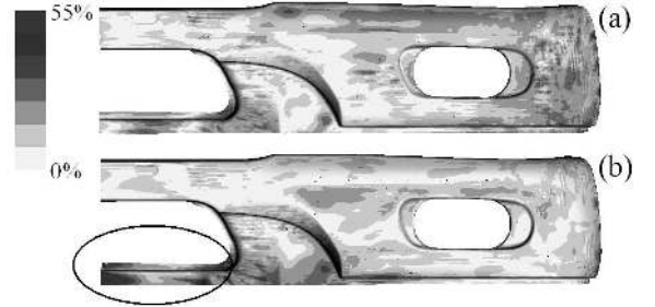
Fig. 12. Iterative (a) and one-step (b) compensation.
