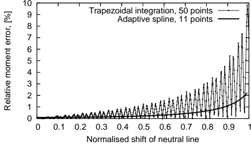
Fig. 7. Relative moment error for various values of in-plane tension obtained with traditional trapezoidal rule and adaptive spline integration.
