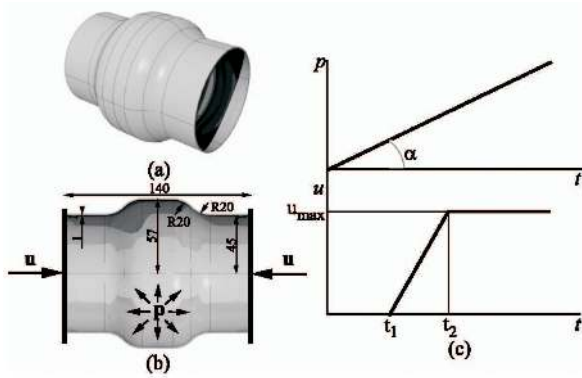
Fig. 20. (a) A simple hydroformed product; (b) Dimensions; (c) Typical load paths for hydroforming.
