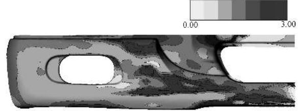
Fig. 11. Local overbending factor on the DAF part.
