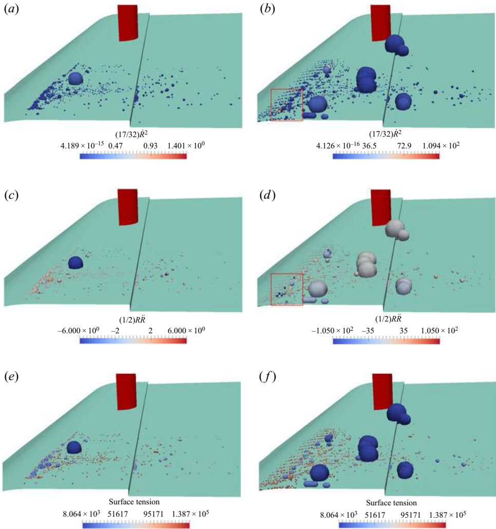
Figure 20. A comparison between inertia and surface tension of bubbles at two instances with low and high vapour volume in the wake area. (a,b) \frac{17}{32}\bar{R}^2 ; (c,d) \frac{1}{2}R\bar{R} ; (e,f) 2\sigma/R . Panels (a), (c) and (e) correspond to figure 19(a); (b), (d) and (f) correspond to figure 19(b). The size of the bubbles are scaled by 40R.
