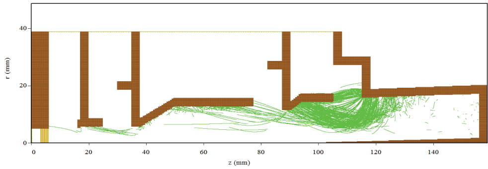
(b) Trajectories of the true secondary electrons
