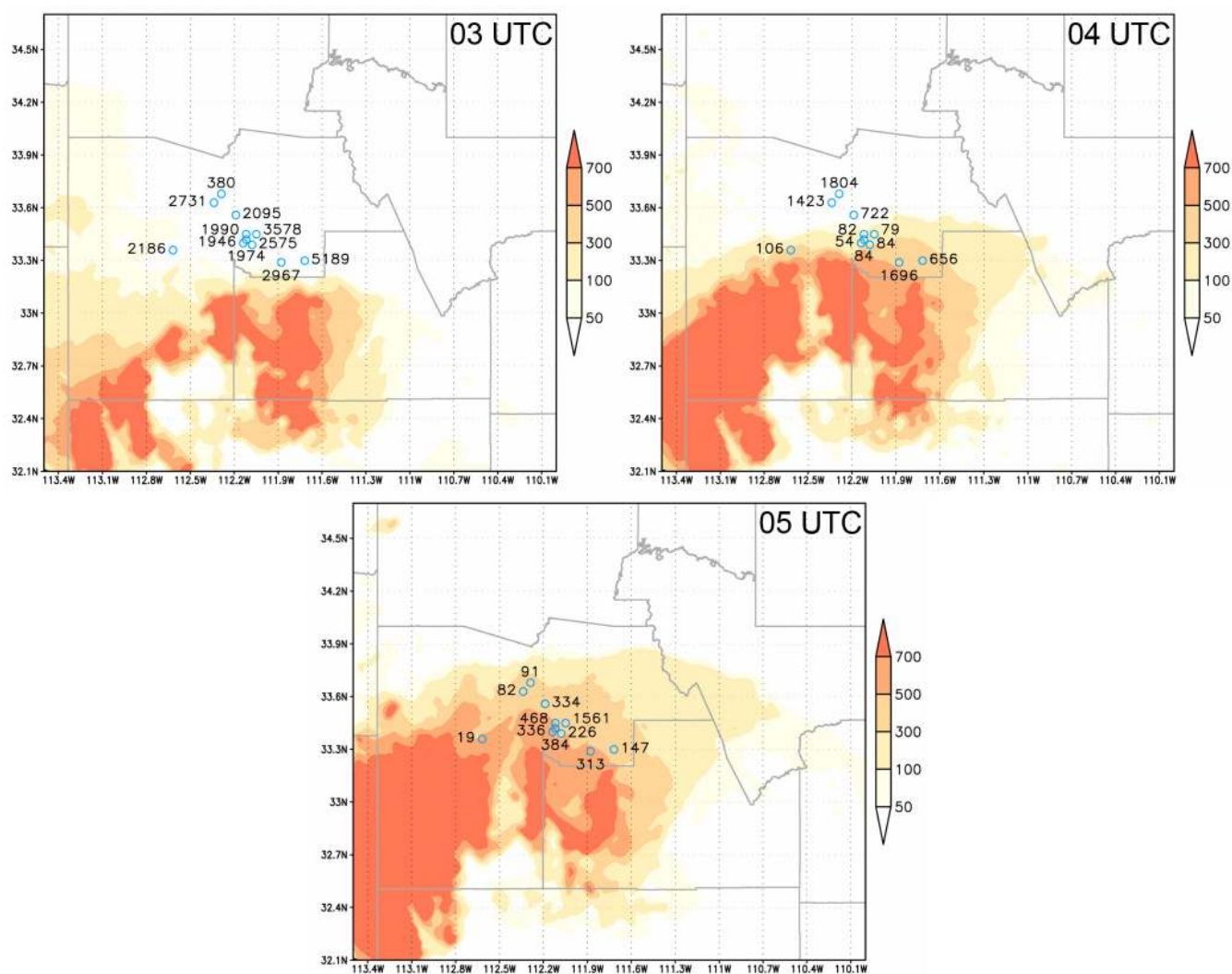
Fig. 9. NMME–DREAM \text{PM}_{10} surface dust concentration and observed values of \text{PM}_{10} ( \mu\text{g m}^{-3} ) at 03:00 (upper left), 04:00 (upper right), and 05:00 (lower) UTC 6 July 2011.
