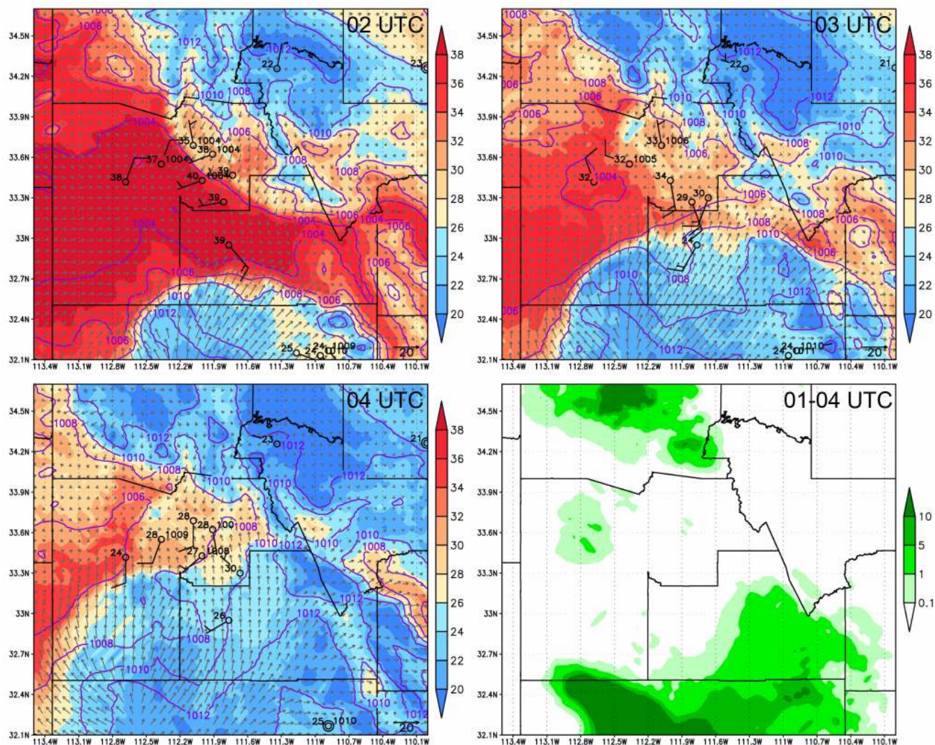
Fig. 5. NMME–DREAM 2 m temperature (blue to red), surface pressure (purple lines) and 10 m wind (arrows), and observed values at stations (2 m temperature, surface pressure and 10 m wind) at 02:00 (upper left), 03:00 (upper right), and 04:00 (lower left) UTC 6 July 2011; NMME–DREAM 3 h accumulated precipitation for the period 01:00–04:00 UTC, respectively, 6 July 2011 (lower right).
