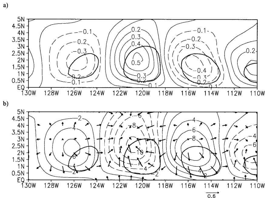
FIG. 4. Close-up of distribution of regression coefficients between 0° and 5°N, 130° and 110°W, model results. (a) Air temperature (at lowest model level, line contours), and SST (thick line contours at + and -0.5). (b) Surface pressure (line contours, Pa K -1 ), SST (thick line contour at + and -0.5 K), and surface wind vectors (m s -1 K -1 ).
