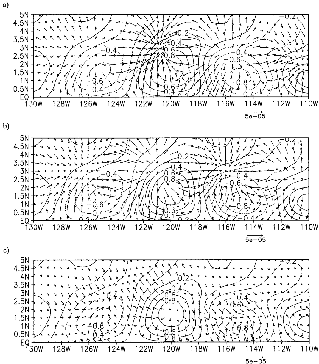
FIG. 8. (a)–(c) Terms in the budget equation for momentum, at bottom model level, regressed onto SST. The terms are shown as vectors, while the regression coefficient of SST is overlaid as contours for reference. Units are \text{m s}^{-2} \text{K}^{-1} . Surface distributions of (a) pressure gradient, (b) vertical mixing, (c) horizontal advection. (d), (e) Longitude section at 2^\circ\text{N} showing combined terms in the (d) U momentum budget and (e) V momentum budget. The combined effects of pressure gradient and vertical mixing (line with open circles) and the total tendency (dashed line with filled symbols) are shown.
