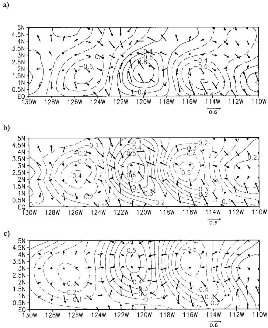
FIG. 3. Close-up of distribution of regression coefficients between 0^{\circ} and 5^{\circ}\text{N} , 130^{\circ} and 110^{\circ}\text{W} . (a) Observed SST (contours) and 10-m neutral equivalent wind vectors ( \text{m s}^{-1} \text{K}^{-1} ), from TMI and QuikSCAT. (b) Observed column-integrated water vapor (contours, \text{mm K}^{-1} ) and 10-m neutral equivalent wind vectors ( \text{m s}^{-1} \text{K}^{-1} ), from TMI and QuikSCAT. (c) Model column-integrated water vapor (contours, \text{mm K}^{-1} ) and 10-m neutral equivalent wind vectors ( \text{m s}^{-1} \text{K}^{-1} ).
