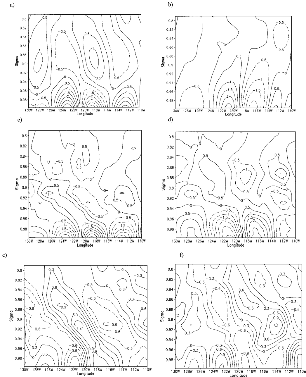
FIG. 9. Vertical cross sections at 2^{\circ}\text{N} of terms in the momentum budget equations, regressed and filtered. (a) For U momentum, the pressure gradient term; (b) V momentum, the pressure gradient term. (c) For U momentum, the vertical mixing term; (d) V momentum, the vertical mixing term. (e) For U momentum, the horizontal advection term; (f) V momentum, the horizontal advection term. Units are \text{m s}^{-2} \text{K}^{-1} .
