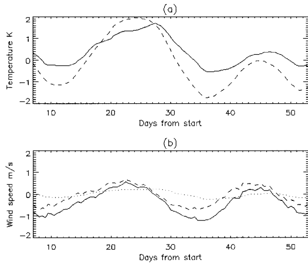
FIG. B1. Effect of static stability on near-surface winds, at 2^{\circ}\text{N} , 120^{\circ}\text{W} . Day 0 refers to 1 Sep 1999. (a) Solid line represents the model-predicted air-sea temperature difference (air temperature at 10 m); dashed line represents SST. (b) Neutral equivalent 10-m wind speed fluctuations. Solid line represents full model predictions. Dotted line represents experiment 1 (see text). Dashed line represents experiment 2 (see text). The data have been smoothed with a running mean over 7 days. (a), (b) The solid lines in have been filtered by removing a 12^{\circ} running mean. The dashed and dotted lines have had the time mean removed.
