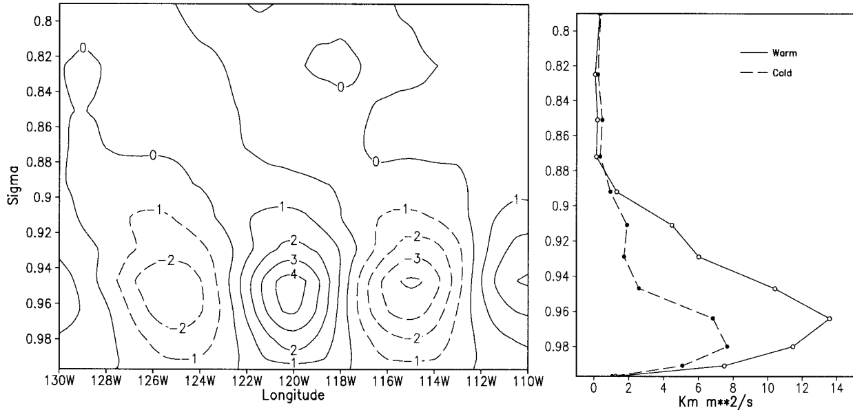
FIG. 6. As in Fig. 5, but for vertical mixing coefficient K_m (line contours, \text{m}^2 \text{s}^{-1} ).
