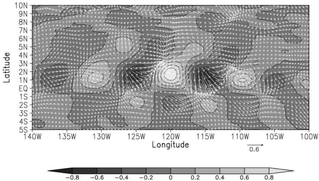
FIG. 2. Regression coefficients of TIW anomalies for a center point at 2°N, 120°W SST (shading) and 10-m neutral equivalent winds (vectors, \text{m s}^{-1} \text{K}^{-1} ). (a) Observations from TMI and QuiKSCAT. (b) Model simulation.
