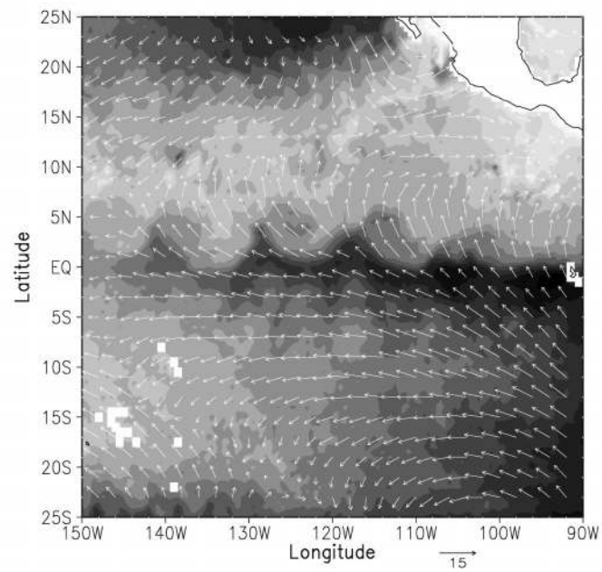
FIG. 1. SST (shading, ^{\circ}\text{C} ) and 10-m neutral equivalent wind vectors ( \text{m s}^{-1} , see scale arrow) over the model domain for a 3-day mean centered on 7 Sep 1999. (a) Observed SST from TMI and wind vectors from QuikSCAT, (b) processed SST data for simulation, with errors replaced with interpolation between good data, and modeled winds over the ocean. Data gaps are shown in white.
