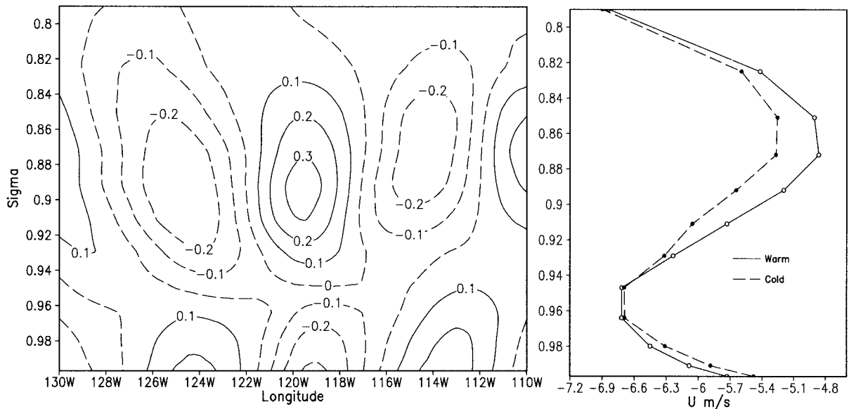
FIG. 5. (left) Regression coefficients (per unit K) in a longitude–vertical plane at 2^{\circ}\text{N} . The vertical coordinate is \sigma , and ranges from the surface to about 2 km height. (right) Accompanying total profiles over warm SST (solid line with unfilled symbols) and over cold SST (dashed line with filled symbols). (a) Virtual potential temperature (K), (b) U velocity ( \text{m s}^{-1} ), (c) V velocity ( \text{m s}^{-1} ), (d) specific humidity \text{g kg}^{-1} with vectors of (u, w \times 100) , ( \text{m s}^{-1} ) overlain.
