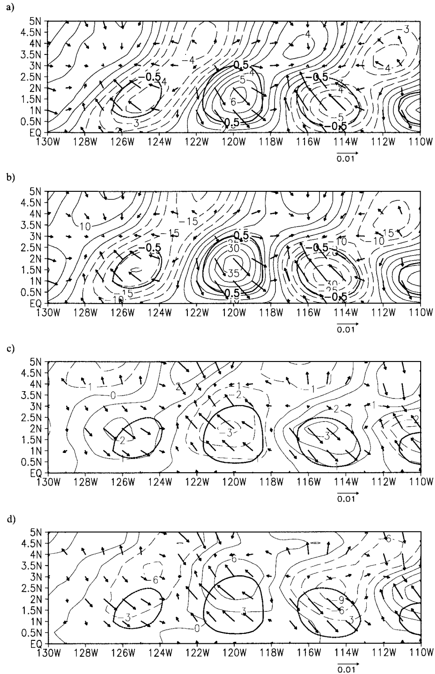
FIG. 7. Regression coefficients of turbulent flux quantities. For reference the SST regression contours of +0.5 , -0.5 are shown as thick black contours. (a), (c) Sensible heat flux SF (line contour, \text{W m}^{-2} \text{K}^{-1} ), and vectors of momentum flux (UF, VF) \text{m}^2 \text{s}^{-2} \text{K}^{-1} . (b), (d) Latent heat flux LF (line contours, \text{W m}^{-2} \text{K}^{-1} ), and vectors of momentum flux (UF, VF) \text{m}^2 \text{s}^{-2} \text{K}^{-1} . (a), (b) At the surface, (c), (d) at \sigma = 0.929 ( \sim 700 m height).
