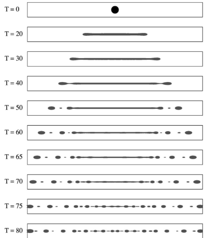
FIG. 16. Interface evolution as viewed from the top of the computational box 12 \times 1 \times 1 during breakup for Ca=0.55 , \lambda=0.77 , equal densities. 256 \times 64 \times 64 grid.
