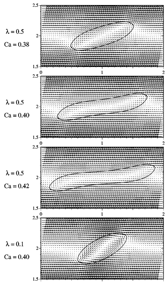
FIG. 10. Cross-sectional slice in x - z plane through the center of the drop. In the top three figures, the viscosity ratio is \lambda=0.5 and Ca=0.38, 0.40, 0.42 . In the bottom plot, \lambda=0.1, Ca=0.40 . The top and bottom solutions have achieved steady states. Equal densities, Stokes flow.
