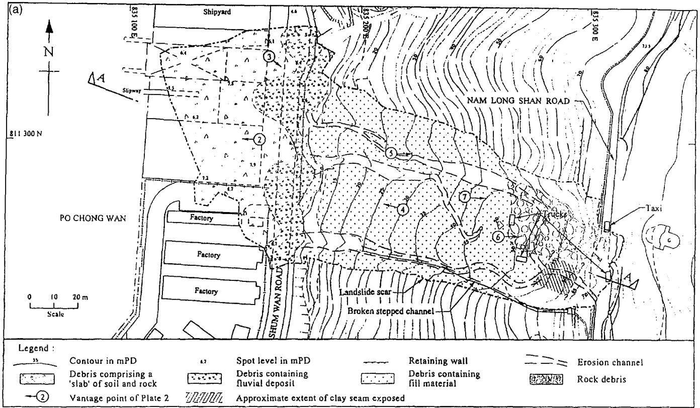
Fig. 3. (a) Plan of the Shum Wan Road landslide, and (b) section A-A through the landslide (for location see a). Information shown in the figure is based on topographic survey, geological mapping, and field observations carried out between 13 August and 23 November 1995.
